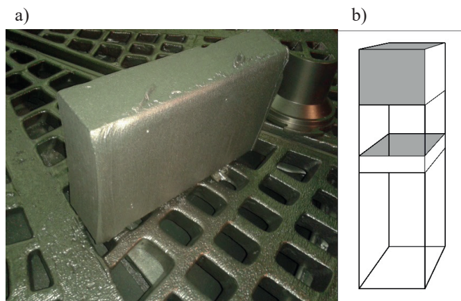
Fig. 1. View of the slab test piece after mechanical cleaning - a) and schematic picture of the specimen cut out from the slab for further metallographic studies - b)
