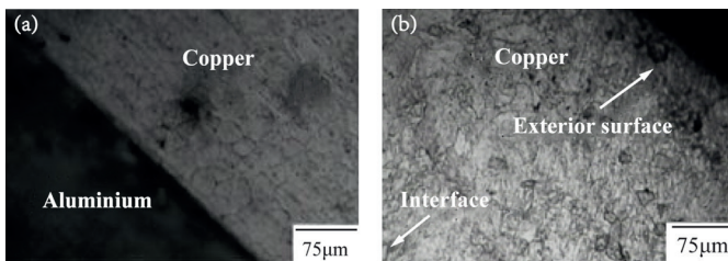
Fig. 5. OM micrograph of copper in cone-shaped deformation zone: (a) Microstructure of copper in interface; (b) Microstructure of copper in surface
