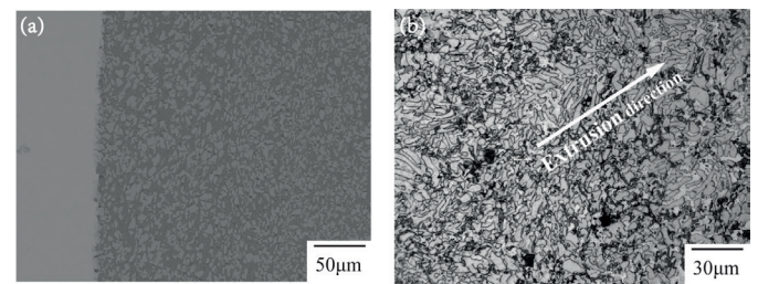
Fig. 6. SEM image of aluminum after extrusion: (a) In radial cross-section; (b) In axial cross-section near the interface
