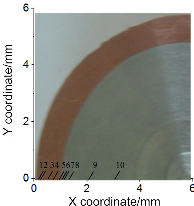
Fig. 7. Radius coordinate diagram of measuring points
