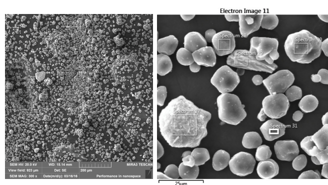
Fig. 3. EDX microscopic analysis of Additive 1
