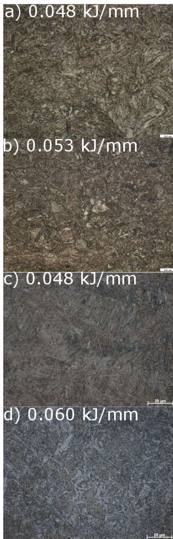
Fig. 6. Microstructure of the heat affected zone of steel TRIP subjected to: a), b) single-spot laser beam welding, c), d) twin-spot laser beam welding
