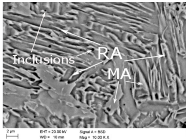
Fig. 5. Microstructure of the fusion zone in steel TRIP subjected to twin-spot laser welding
