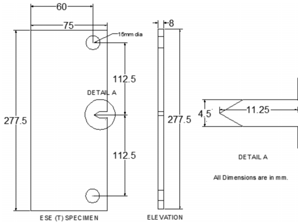
Fig. 1. Deatails of ESE(T) specimen
