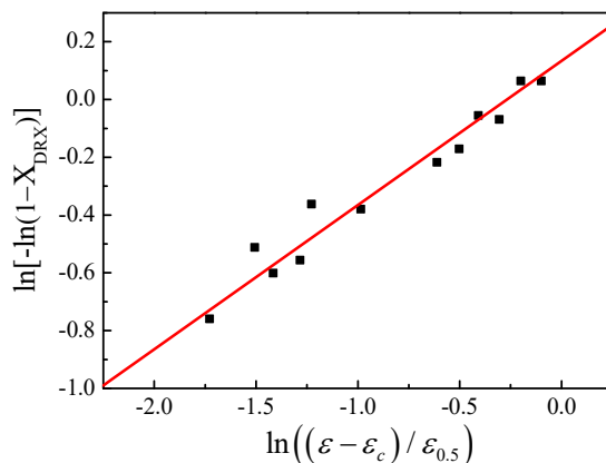
Fig. 12. The relationships between \ln[-\ln(1 - X_{DRX})] and \ln[(\varepsilon - \varepsilon_c)/\varepsilon_p]
