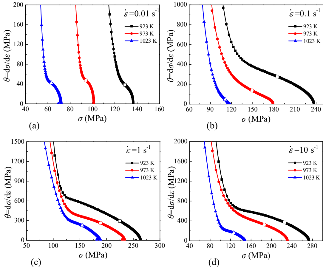
Fig. 9. d\sigma/d\epsilon versus \sigma plots up to the peak points of the true stress-strain curves under different deformation temperatures with strain rates (a) 0.01\text{ s}^{-1} , (b) 0.1\text{ s}^{-1} , (c) 1\text{ s}^{-1} , (d) 10\text{ s}^{-1}
