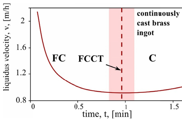
Fig. 5b. Situation of the FCCT as suggested by the local minimum of the function presenting the liquidus velocity of movement versus time
