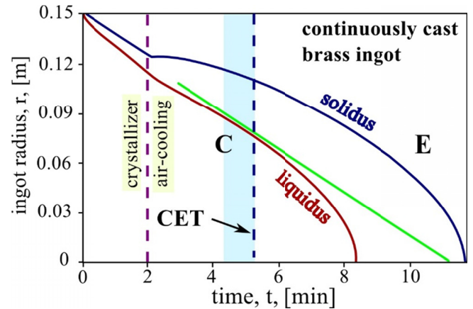
Fig. 4a. Forecast of the CET – transformation for a given rate of brass ingot movement in the crystallizer (equal to 0.4 [m/min]), as suggested by the local maximum in the STSM (Space-Time-Structure Map)
