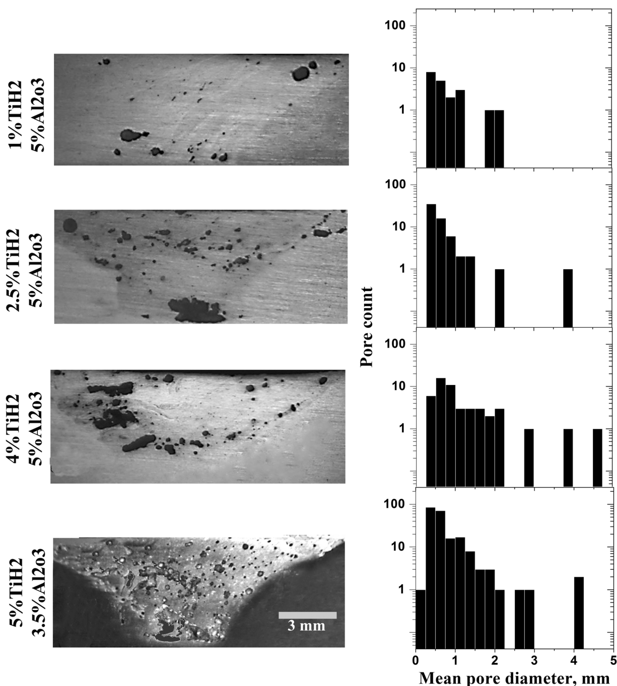
Fig. 3. Effect of the \text{TiH}_2 to \text{Al}_2\text{O}_3 weight ratio on the pore size and distribution in the 4 pass FSP samples fabricated at 858 K
