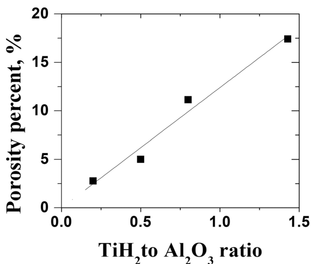
Fig. 5. Variation of porosity in the FSP samples processed with the \text{TiH}_2 to \text{Al}_2\text{O}_3 weight ratio
