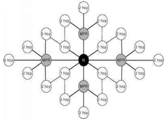
Fig 1. MPR Mechanism
