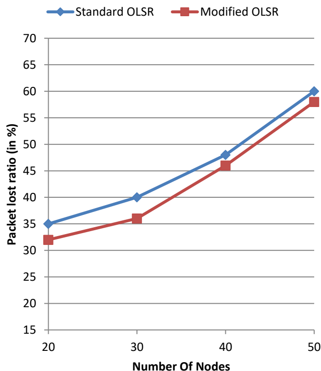
Fig. 4. Packet Lost Ratio.
