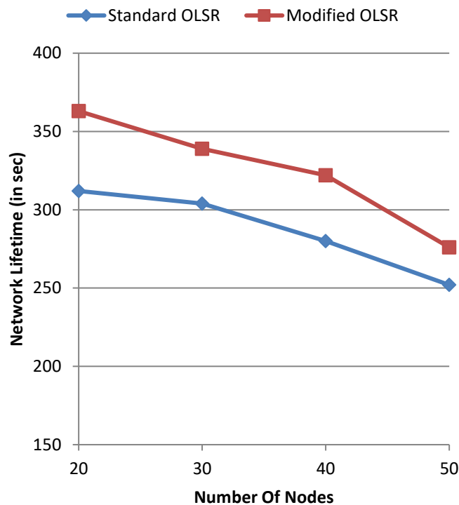
Fig. 3. Network Lifetime
