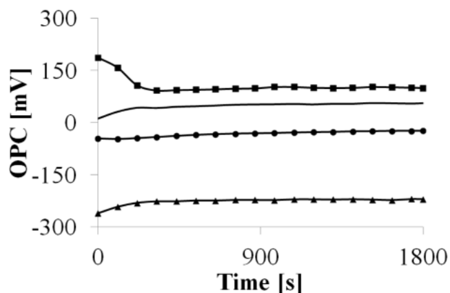
Fig. 2. Open circuit potential ( E_{\text{OCP}} ) of TNT/ \text{H}_3\text{PO}_4 (circle), TNT/ \text{H}_3\text{PO}_4/\text{Ar} (square), TNT/GLY (up triangle) and TNT/GLY/Ar (solid line) measured in 0.01 M PBS for 30 min
