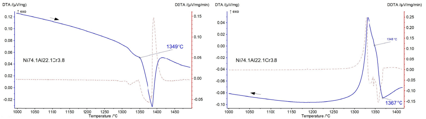
Fig. 10. DTA curves registered during heating (left) and cooling (right) of alloy Ni74.1Al22.1Cr3.8 (20°C/min)
