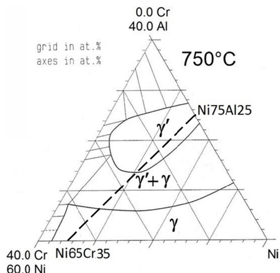
Fig. 1. Isothermal section of Ni-rich part of Ni-Al-Cr system at temperature 750°C proposed by Taylor and Floyd [9]. Broken line shows Ni75Al25÷Ni65Cr35 section with chemical composition representing alloys studied in this work
