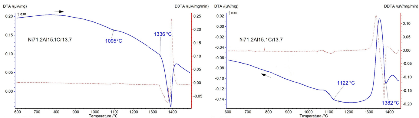
Fig. 7. DTA curves registered during heating (left) and cooling (right) of alloy Ni71.2Al15.1Cr13.7 (20°C/min)
