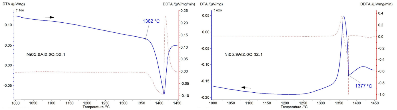
Fig. 2. DTA curves registered during heating (left) and cooling (right) of alloy Ni 65.9 Al 2.0 Cr 32.1 (20°C/min)
