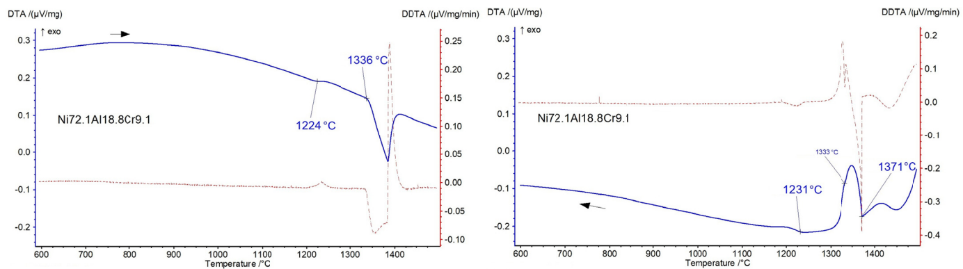
Fig. 8. DTA curves registered during heating (left) and cooling (right) of alloy Ni72.1Al18.8Cr9.1 (20°C/min)
