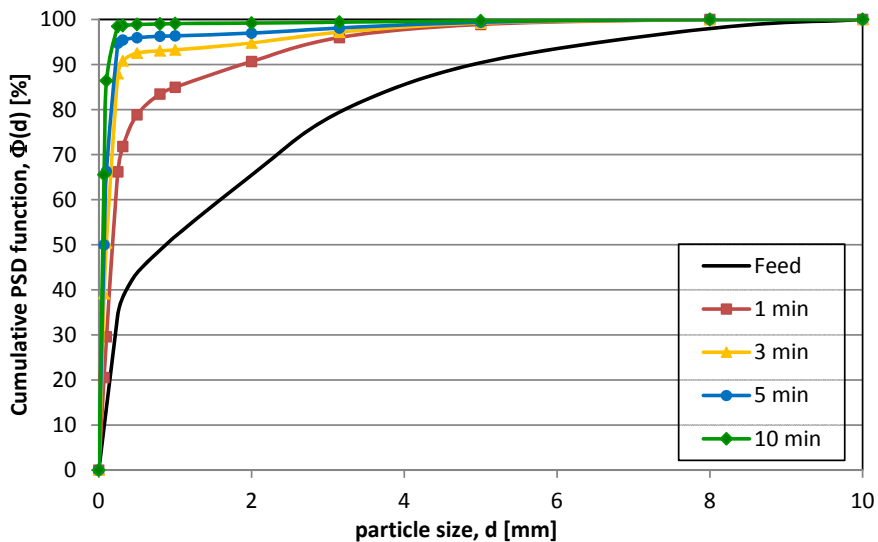
Fig. 5. PSD's of ball mill products for a prior comminution in HRC at 3.5 N/mm 2
