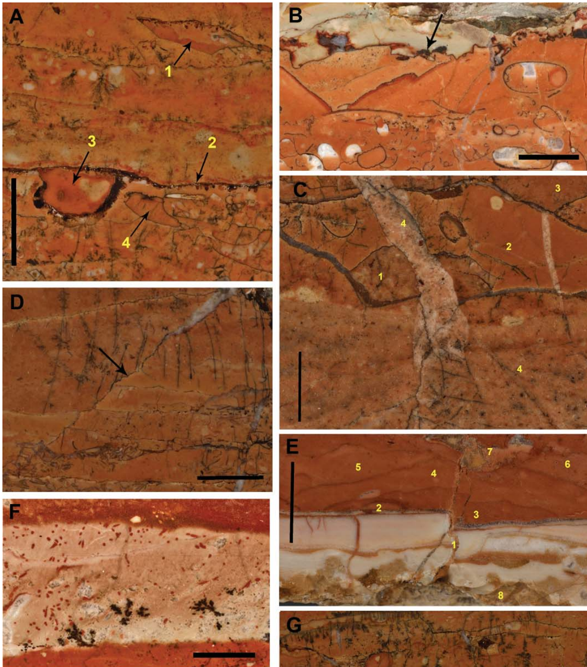
Text-fig. 7. Close-ups of polished vertical sections of neptunian sills. A–D, F–G from RB 18. A. Boundary between units 6 and 7. 1 = reworked clast from lower level, 2 = Fe/Mn-stained boundary, 3 = erosional remnant, 4 = reworked ammonite. B. Boundary between units 15 and 16 marking major gap with erosional surface (arrowed). C. Top of unit 13 showing subsequent depositional stages (1–3), separated by high-angle unconformities, cross-cut by sedimentary dyke (4). D. Oblique, erosionally overprinted normal fault (arrowed) in unit 9. E. Base of main neptunian dyke in section RB 50 (lower Toarcian), fragmented by minor fault (1) and small fissures, overlain by unconformable layers of mudstone (2–7) and underlain by later (probably Oxfordian) neptunian sill (8). F. Fucoid burrowings in topmost level of unit 17. G. Small normal fault (arrowed) off-setting erosional surface in unit 9. All scale bars = 1 cm
