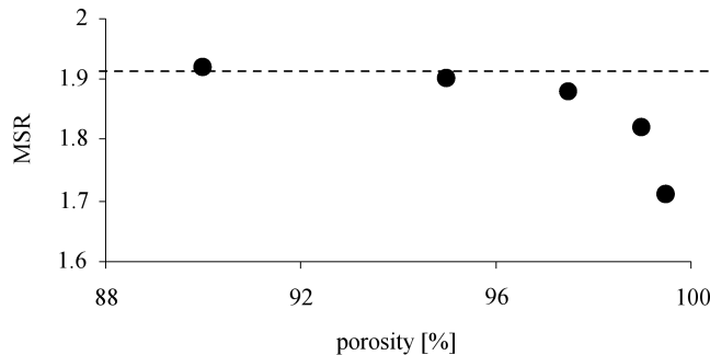
Fig. 4. The dependence between the MSR factor and structural porosity ( d = 0.12 mm). The dashed line corresponds to the MSR value = 1.91.
