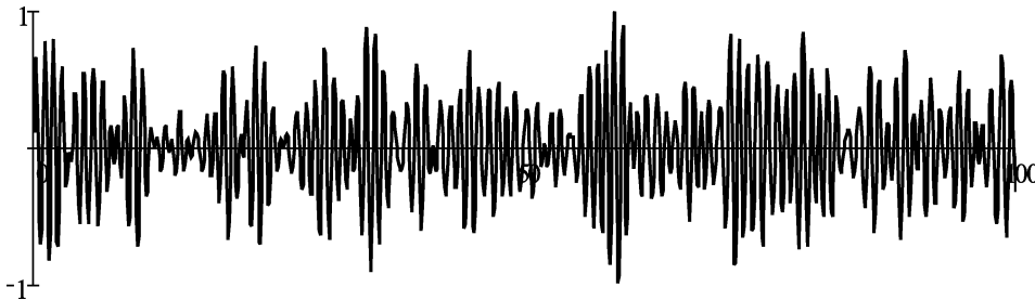
Fig. 3. An example of 1MHz RF-echo simulated for the trabecular bone model consist of identical cylinders ( d = 0.12 mm, \rho = 1900 kg/m 3 , v = 3800 m/s).
