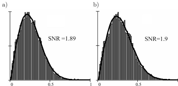
Fig. 5. The histograms of normalized amplitudes of backscattered signals simulated for two structures, substantially different in velocity value of trabeculae material: a) – v = 3800 \text{ m/s} , b) – v = 3200 \text{ m/s} . The continuous line corresponds to the Rayleigh distribution. Porosity – 97.5%.
