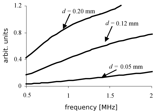
Fig. 2. Frequency dependent backscattering coefficient for a cylinder calculated with varying diameter d = 0.2, 0.12 and 0.05 mm and constant velocity c = 4 \times 10^3 m/s and density \rho = 1900 kg/m 3 .
