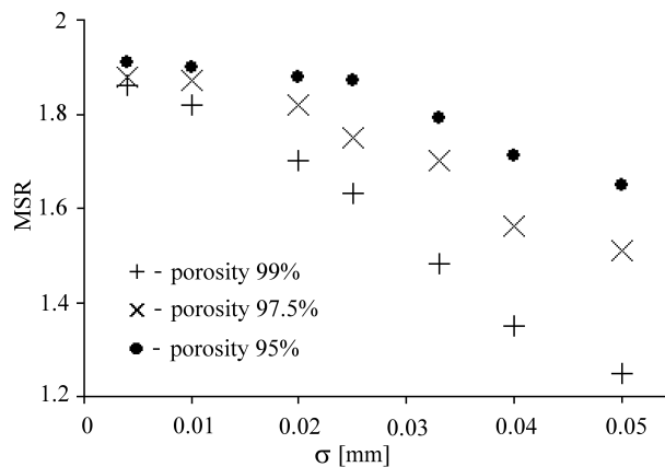
Fig. 7. The MSR factor calculated using the envelopes of signals that are backscattered in the trabecular structure. Thickness of trabeculae is Gamma distributed with the mean equal 0.05 and variable value of standard deviation ( \sigma ).
