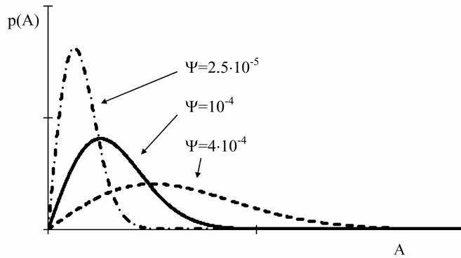
Fig. 1. Rayleigh probability density function for various values of the \Psi parameter.
