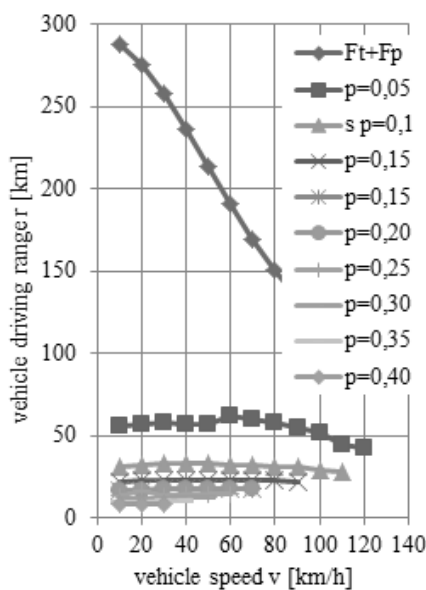
Fig. 9. The characteristic curve of a vehicle's driving range (overcoming grade resistance): F_t + F_p – sum of rolling resistance and air resistance, p – slope
