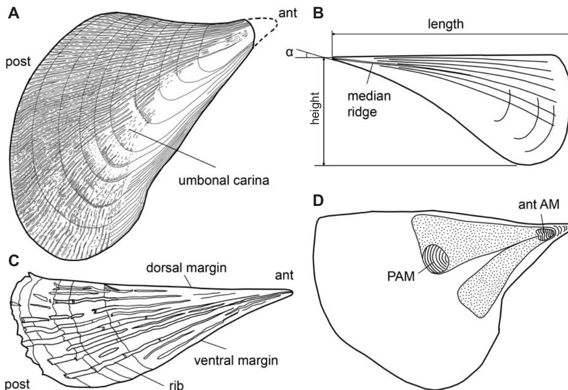
Text-fig. 3. Orientation and terminology. A – Stegoconcha ampla (J. Sowerby, 1812), right valve (RV), modified after holotype figure; Middle Jurassic, England; B – Pinna (Cyrtopinna) sp. , Upper Jurassic, left valve (LV), \alpha – umbonal angle; C – Pinna (P.) rudis Linnaeus, 1758; Recent, Barbados; ant – anterior, post – posterior; D – Pinna (Exitopinna) deltodes Menke, 1843; Recent, Australia; left valve interior, stippled fields – lobes of nacre, PAM – posterior adductor muscle scar, ant AM – anterior adductor muscle scar
