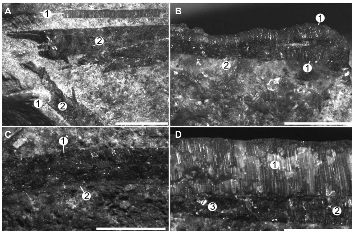
Text-fig. 5. Stegoconcha plotii (Arkell, 1933). FPJ 21621, Lower Callovian (Ifenthal Formation, Châtillon Member) of the “Tunnel de Choindez” (A 16), Switzerland, natural cross-sections. A – dorsal margin of articulated valves (LV up), 1, calcitic, regular simple prismatic outer shell layer, 2, internal aragonitic nacreous shell layer (recrystallised), B – anteroventral margin of RV, 1, folded calcitic, regular simple prismatic shell layer (SP), 2, nacreous internal shell layer, C – longitudinal cut, middle of shell, 1, continuous aragonitic nacreous shell layer (not divided into lobes), 2, thin aragonitic prismatic shell layer, D – longitudinal cut, posterior end, 1, calcitic, regular simple prismatic outer shell layer, 2, internal probably calcitic simple prismatic layer, 3, aragonitic nacreous layer (grading into 2 in posterior direction). Scale bars equal to 5 mm (A) and 3 mm (B-D)
