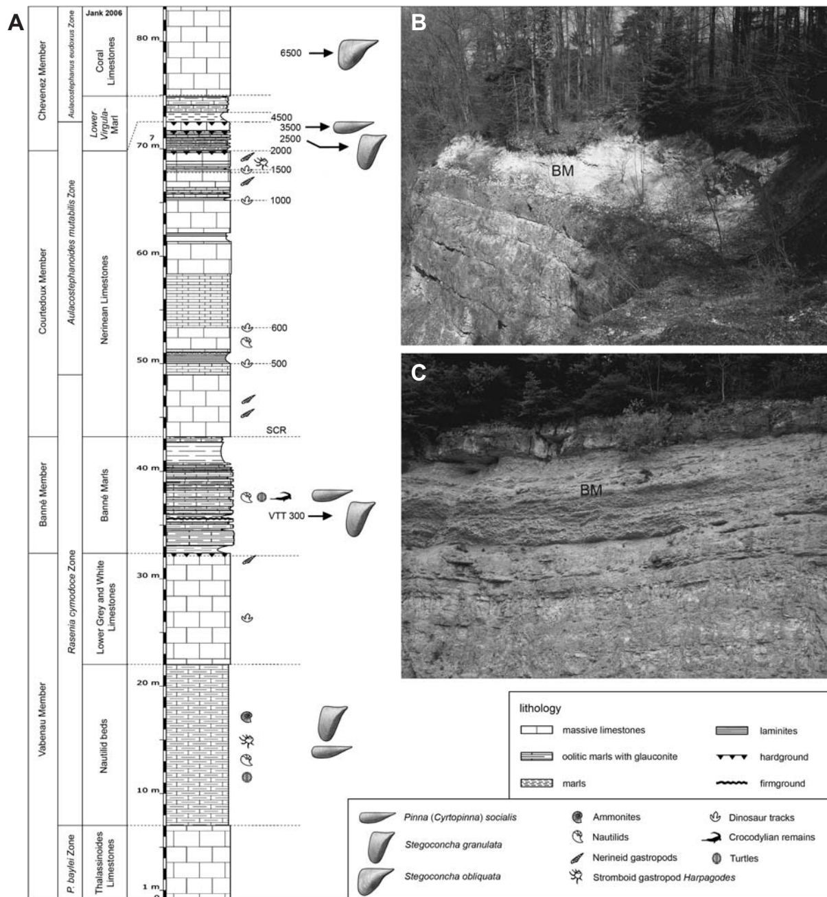
Text-fig. 2. A – Generalised section of the Reuchenette Formation in the Ajoie area (based mainly on the Vâ tche Tchâ, VTT and Sur Combe Ronde, SCR sections); B – Banné Marls (c. 5 m in thickness) in the abandoned Vendlincourt-Ecochevez quarry (VEN-ECO), C – Banné Marls (c. 6 m) in Alombre aux Vaches; BM – Banné Marls
