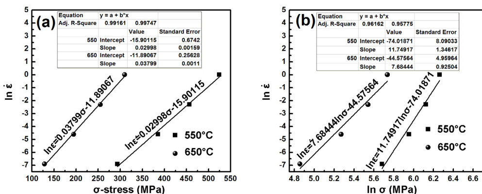
Fig. 4. Relationships between (a) \ln \dot{\varepsilon} and \sigma , and (b) \ln \dot{\varepsilon} and \ln \sigma
