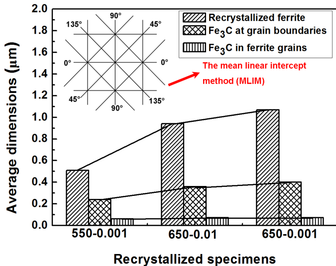
Fig. 12. The size of ferrite grains and \text{Fe}_3\text{C} particles in completely recrystallized specimens
