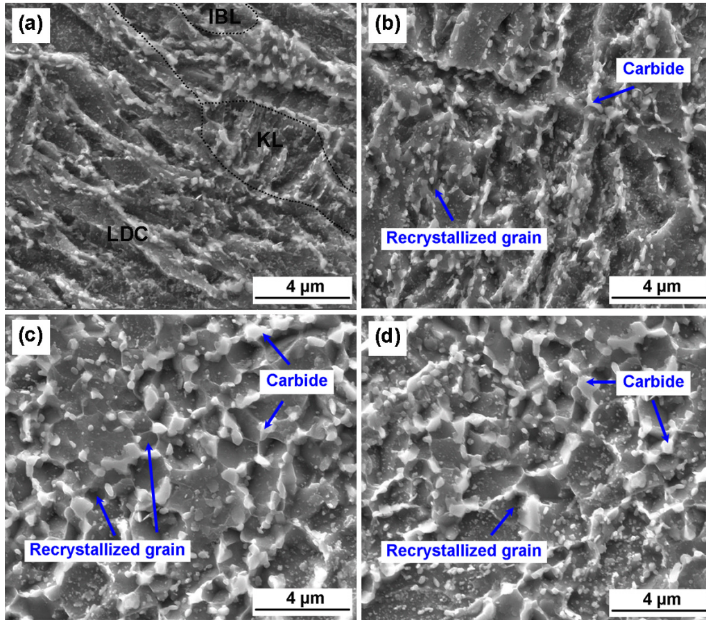
Fig. 11. Microstructures in specimens after warm deformation at 650°C with different strain rates: (a) 1 \text{ s}^{-1} ; (b) 0.1 \text{ s}^{-1} ; (c) 0.01 \text{ s}^{-1} and (d) 0.001 \text{ s}^{-1}
