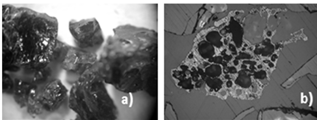
Fig. 5. GCFS (magnification 2.5\times ) – a and its microstructure ( 100\times ) – b
