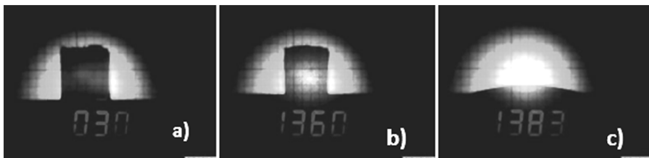
Fig. 3. Course of GBFS sample melting
