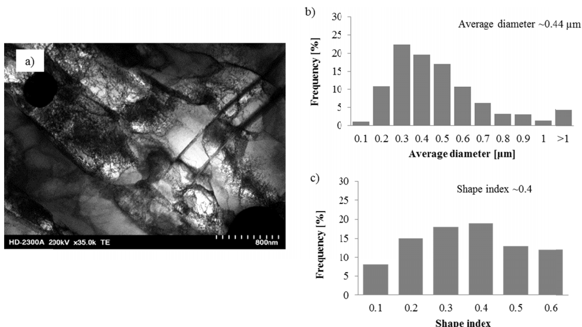
Fig. 4. Microstructure of CuCr0.6 alloy for S1+COT a), distribution of average grain/subgrain size b) distribution of shape index
