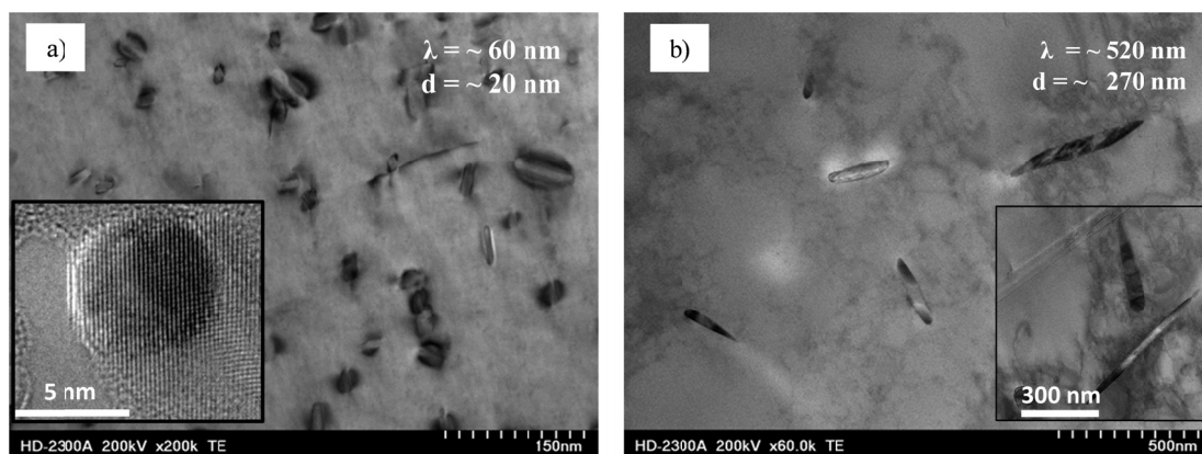
Fig. 3. Microstructure of CuCr0.6 alloy after S1 a), and microstructure of CuCr0.6 alloy after S2 b)
