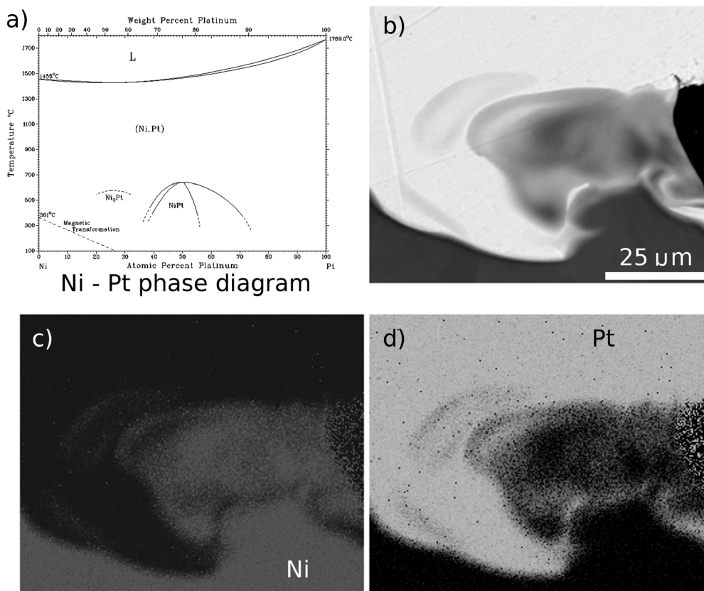
Fig. 4. a) the Ni-Pt phase system; b) the microstructure of Inconel 625/Pt joint in the central part of the fusion zone; c) nickel distribution in the weld; d) platinum distribution in the weld
