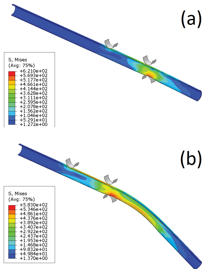
Fig. 12. The distribution of Mises (HMH) equivalent stress for the laser-assisted tube bending: (a) t = 20.0 s, (b) t = 120.0 s
