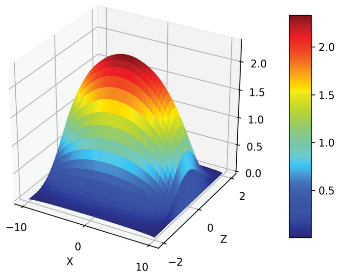
Fig. 8. Distribution of radiation surface intensity [ \text{W}/(\text{mm}^2) ] in the local reference frame of the laser spot
