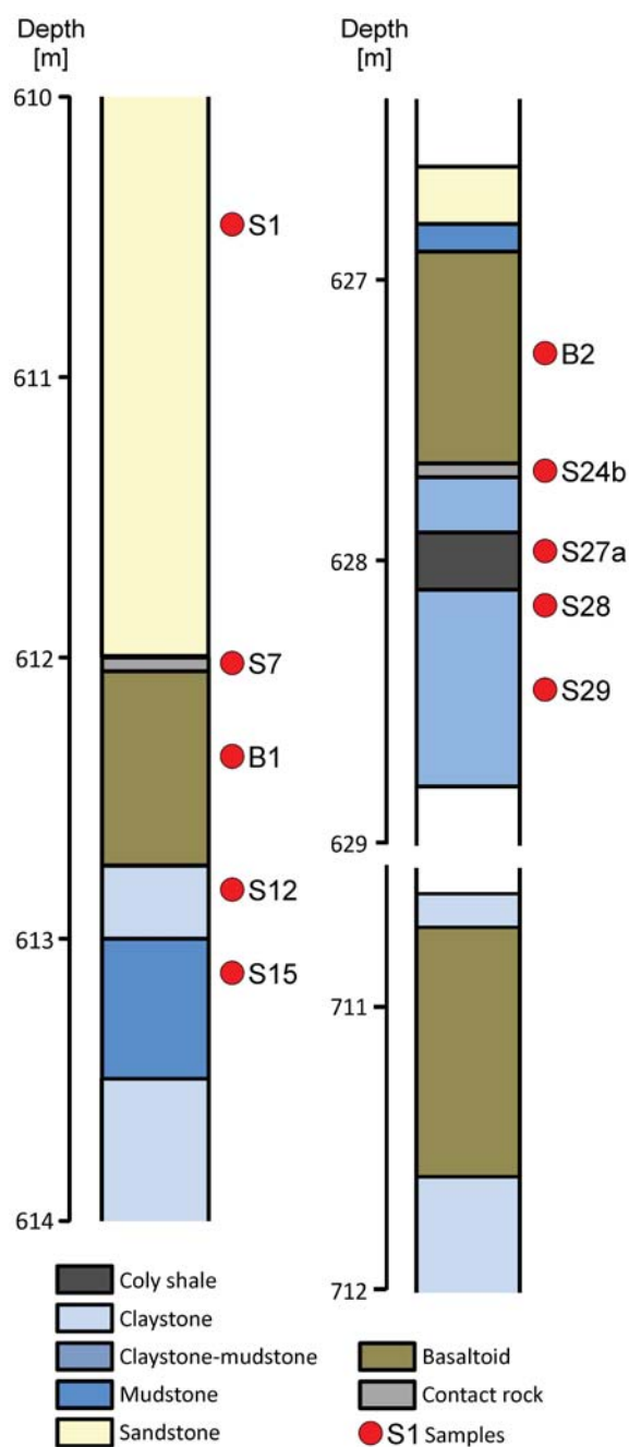
Text-fig. 3. Samples localization in the geological profile of the Sumina S-7 (USCB) with basaltoid intrusions
