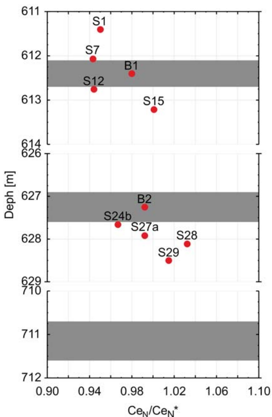
Text-fig. 16. Distribution of Ce anomaly value in the profile of the Sumina S-7
