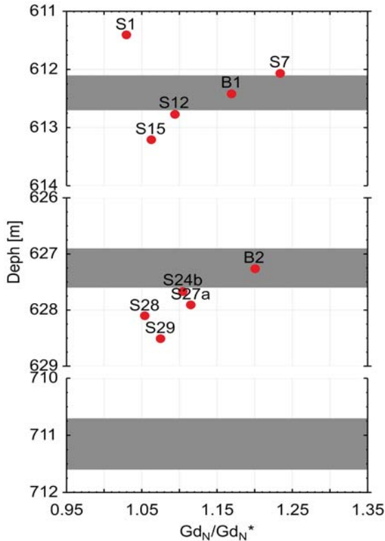
Text-fig. 12. Distribution of Gd anomaly value in the profile of the Sumina S-7
