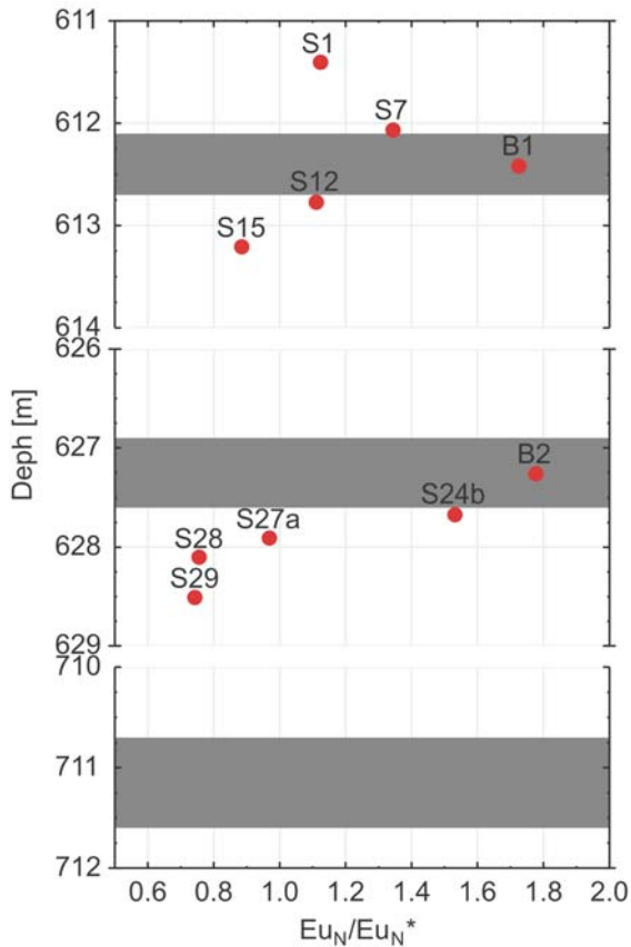
Text-fig. 10. Distribution of Eu anomaly value in the profile of the Sumina S-7
