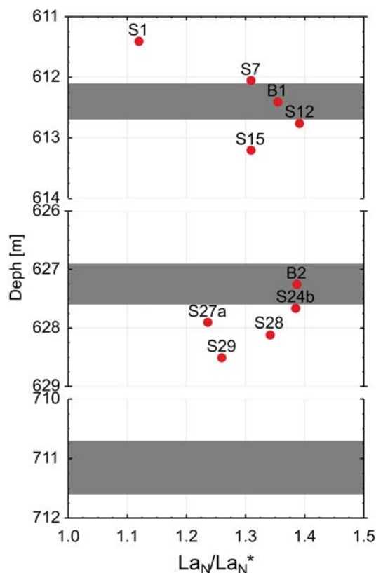
Text-fig. 14. Distribution of La anomaly value in the profile of the Sumina S-7
