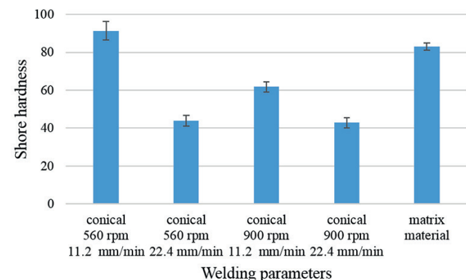
Fig. 15. The results of Shore hardness of welded joints prepared by conical pin
