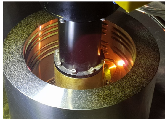
Fig. 1. Rotating direct-metal deposition experiments on cylinder inner wall
