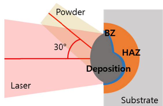
Fig. 2. Asymmetric dilution in non-coaxial rotating direct-metal deposition. BZ: bonding zone; HAZ: heat-affected zone
