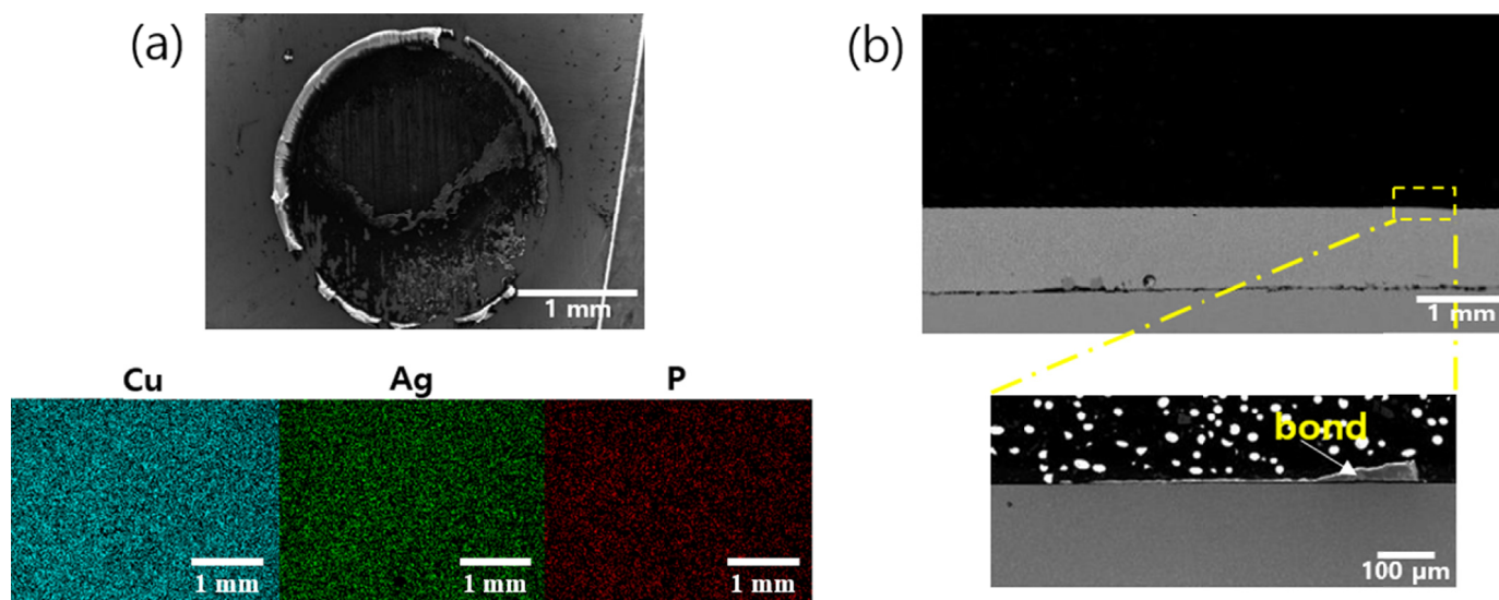
Fig. 7. SEM observation results of pull out specimen (a) surface image and (b) cross-sectional images
