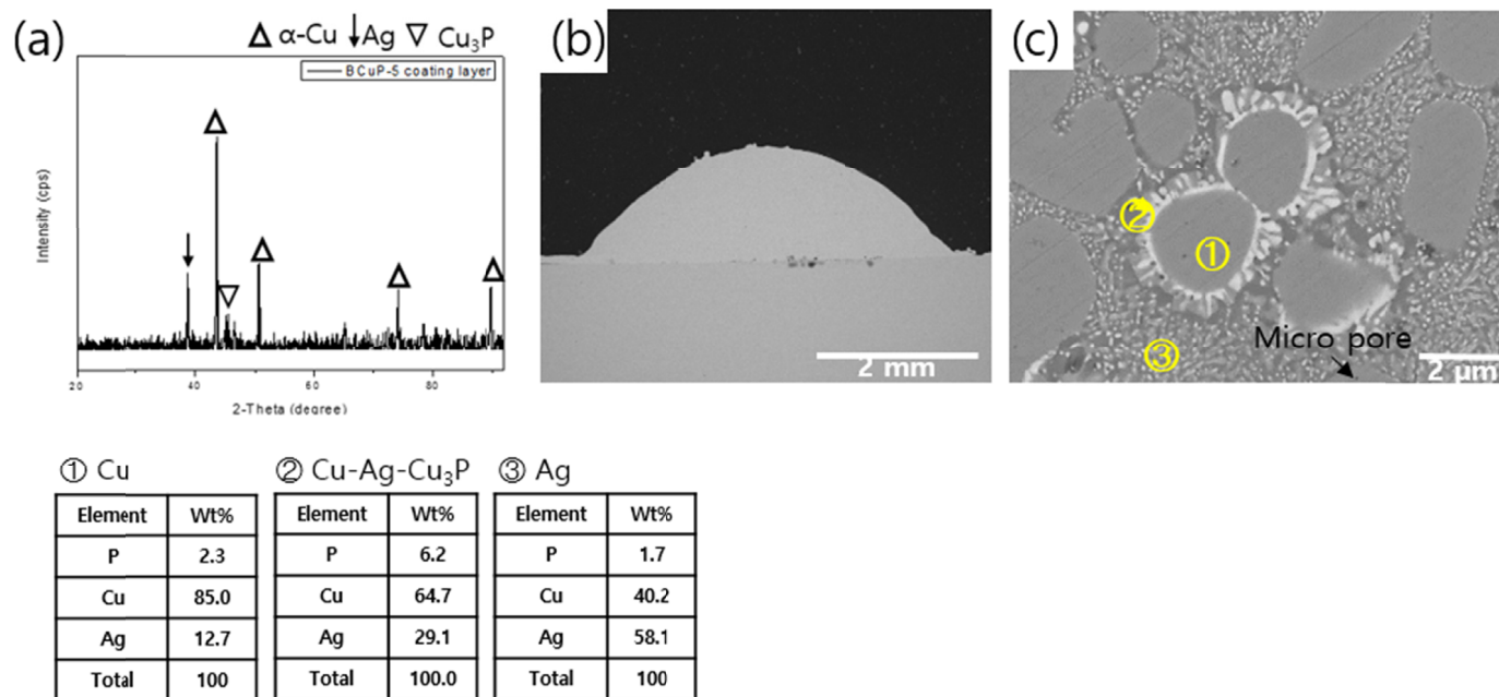
Fig. 4. Results of coating layer observation (a) XRD and (b, c) SEM/EDS
