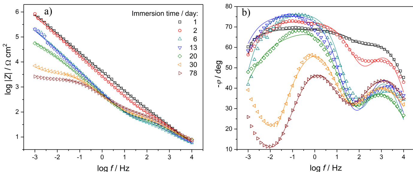
Fig. 5. Experimental (symbol) and approximated (line) Bode diagrams in the form of \log|Z| = f(\log f) a) and \varphi = f(\log f) b) for the Ti15Mo electrode in saline solution after different immersion time at 37°C
