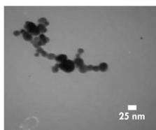
TEM image of Co 3 O 4 NPs
