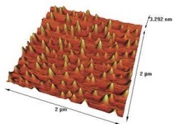
AFM image of Co 3 O 4 NPs
