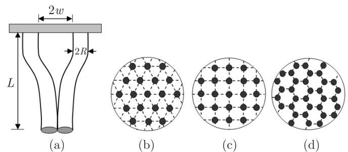
Fig. 4. Anti-bunching condition of a fibrillar structure. (a) Configuration of self-bunching in an array of fibres distributed in (b) triangular, (c) square or (d) hexagonal patterns
