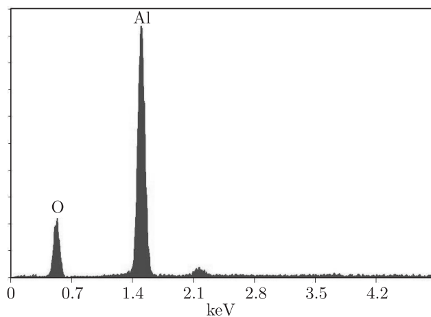
Fig. 8. The energy dispersive spectrum (EDS) of the fibers fired at 1500°C/1h
