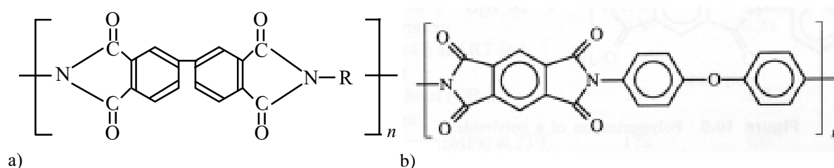
Fig. 6. Structure of high-temperature polyamide foil UPILEX® a) and KAPTON® b), examined during the research
