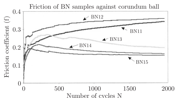
Fig. 12. Dependence of friction coefficient from number of cycles obtained during "ball-on-disk" wear test of BN/Ti x N/Ti6Al4V specimens
