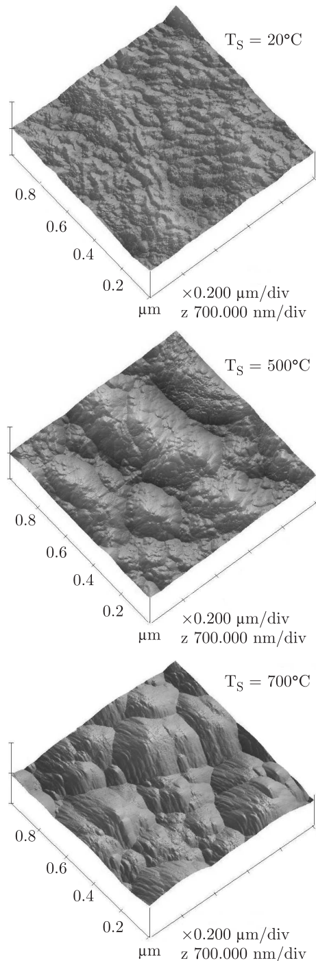
Fig. 6. AFM images (area 1 \times 1 \mu\text{m} ) of the surface of the samples obtained on nitrated Ti6Al4V alloy at substrate temperature of 20°C, 500°C or 700°C and with the fluence of 14 \text{ J/cm}^2 and nitrogen pressure of 5 Pa
