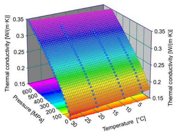
Fig. 8. Thermal conductivity k of the Camelina sativa oil, as a function of pressure p and temperature T .
