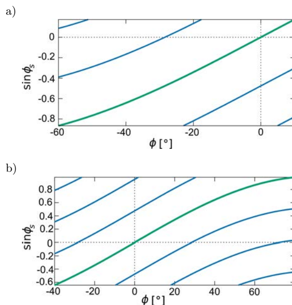
Fig. 30. The diagrams of shifted sine curves for different ranges of angles \phi and their corresponding ranges of sine values: a) \Phi = [-60^\circ, 10^\circ] , b) \Phi = [-40^\circ, 80^\circ] .
