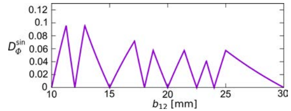
Fig. 32. The dependence of D_{\Phi}^{\sin} on the values of b_{12} when b_{01} = 30 mm.
