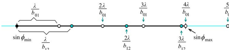
Fig. 34. Two sequences of the solution values of Eq. (3) generated by receiver pairs (R_0, R_1) and (R_1, R_2) for the azimuth angle \phi_{\min} .
