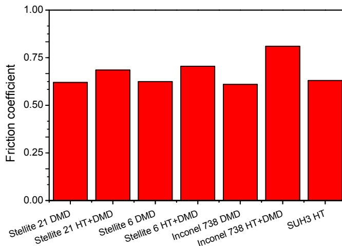
Fig. 3. Friction coefficient results
