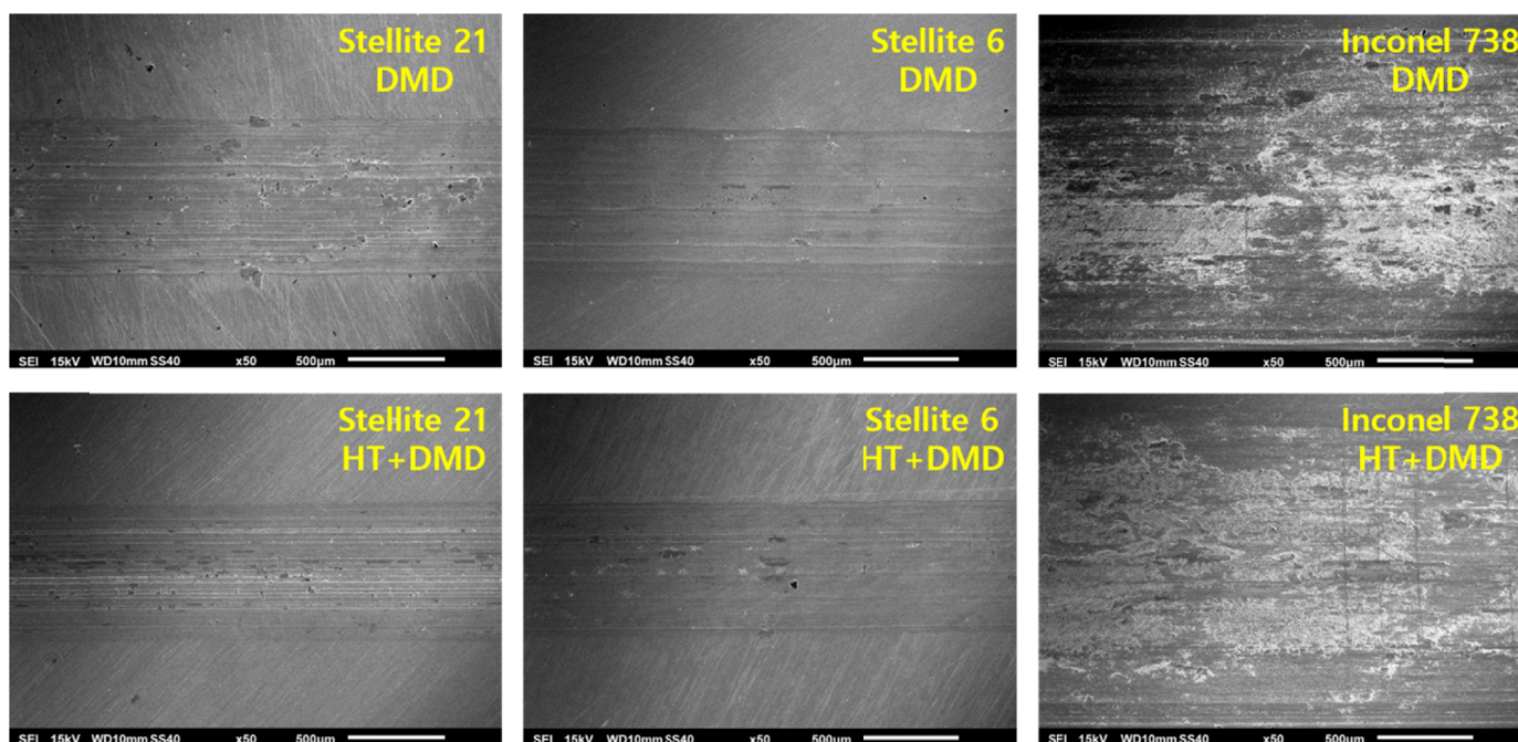
Fig. 4. Wear tracks
