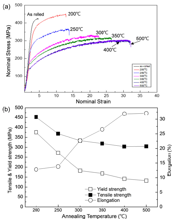
Fig. 5 Nominal stress-strain curves (a) and the mechanical properties (b) of the specimens annealed at various temperatures
