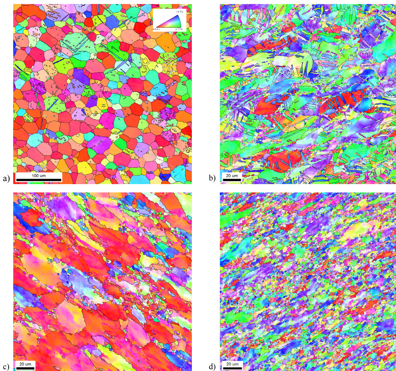
Fig. 3. Orientation distribution maps made for samples from the MgLi1Ca0,2Zn1 alloy cross-section after a) extrusion, b) 1 st pass of ECAE, c) 2 nd pass of ECAE and d) after the 3 rd pass of ECAE
