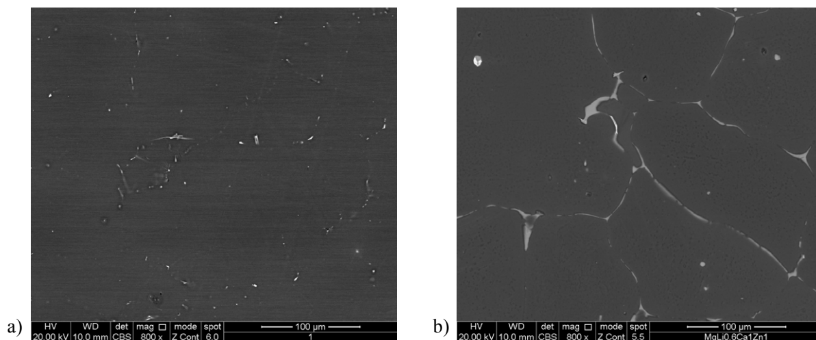
Fig. 1. The structure of alloys: a) MgLi1Ca0,2Zn1 and b) MgLi1Ca1Zn1 after casting
