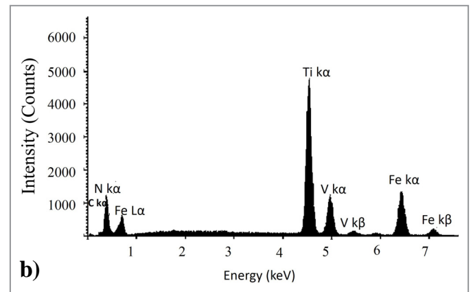
Fig. 10. (a): SEM image and (b): EDS analysis of the titanium precipitate
