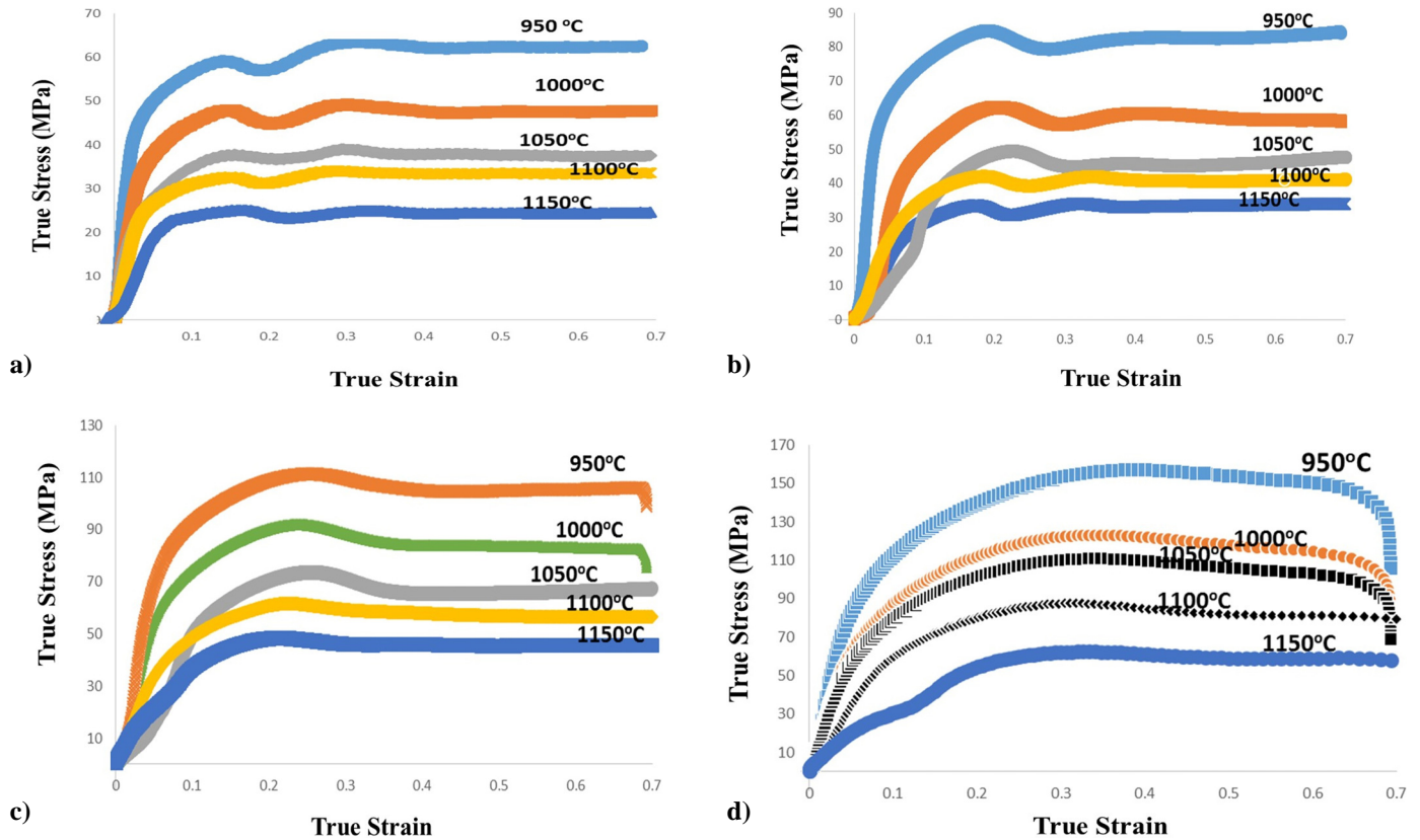
Fig. 2. Flow stress-strain curves at various temperatures and strain rates: (a) 0.001 \text{ s}^{-1} , (b) 0.01 \text{ s}^{-1} , (c) 0.1 \text{ s}^{-1} , (d) 1 \text{ s}^{-1}
