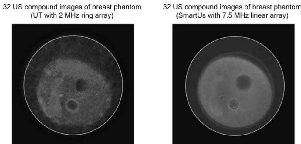
Fig. 6. The comparison between images obtained as in Fig. 4 but after the FASCI reconstruction of 32 sectoral images acquired around the phantom (courtesy of DRAMIŃSKI S.A. company).
