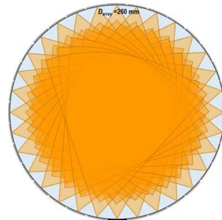
Fig. 2. Illustration of the FASCI reconstruction scheme of 2-D coronal section image using sectoral images obtained by linear phased scanning with ultrasound tomography multi-element ring array.
