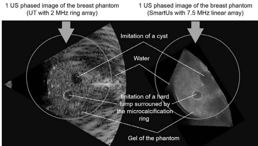
Fig. 4. Images of the same coronal section fragment of the Model B-MM – 1.2 Yezitronix breast phantom obtained by means of the 32-element subarray of the ultrasound tomography ring array (2 MHz) with linear phased mode scanning, and by means of the conventional linear array (7.5 MHz) of the SmartUs Telemed B-mode scanner with virtual convex scanning (courtesy of DRAMIŃSKI S.A. company).
