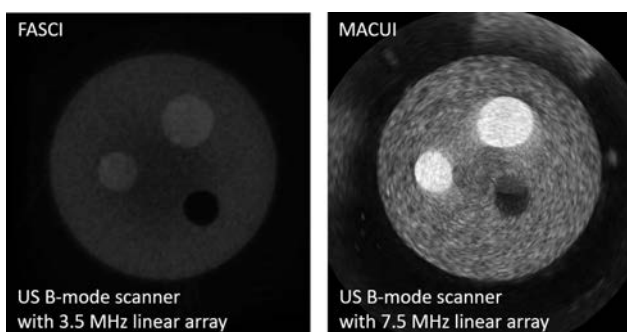
Fig. 18. The images of the same coronal section of an agar gel phantom dipped in water, obtained using FASCI and MACUI method.
