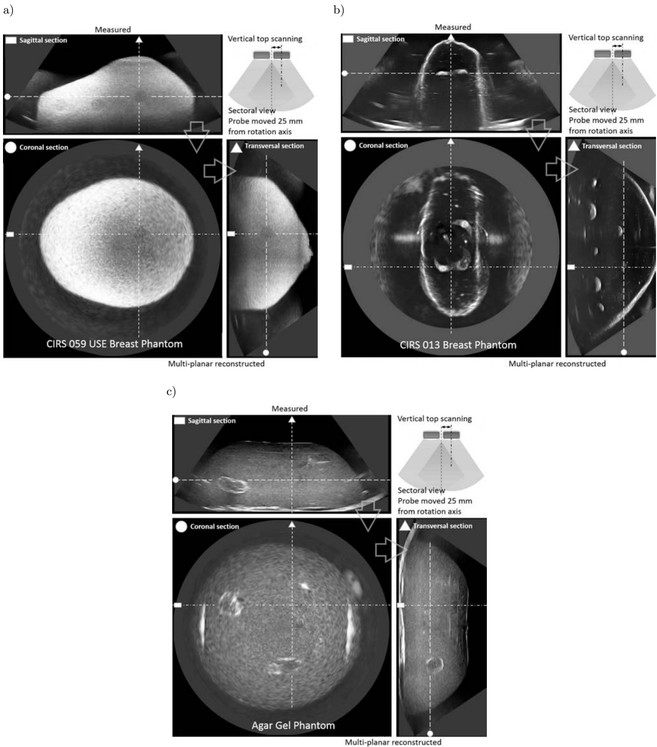
Fig. 15. Images of selected breast phantom sections acquired using vertical top scanning with the sectoral view and the probe moved 25 mm from rotation axis: a) CIRS Model 059 USE Phantom, b) CIRS 013 Mammography Phantom, c) self-made Agar Gel Phantom.
