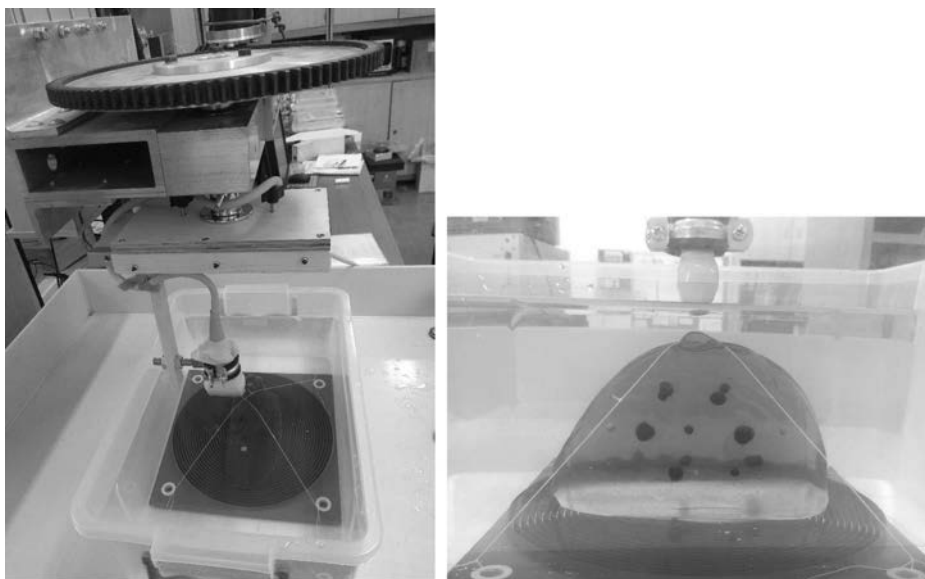
Fig. 8. Measurement system used in multi-angle conventional ultrasound imaging (MACUI).
