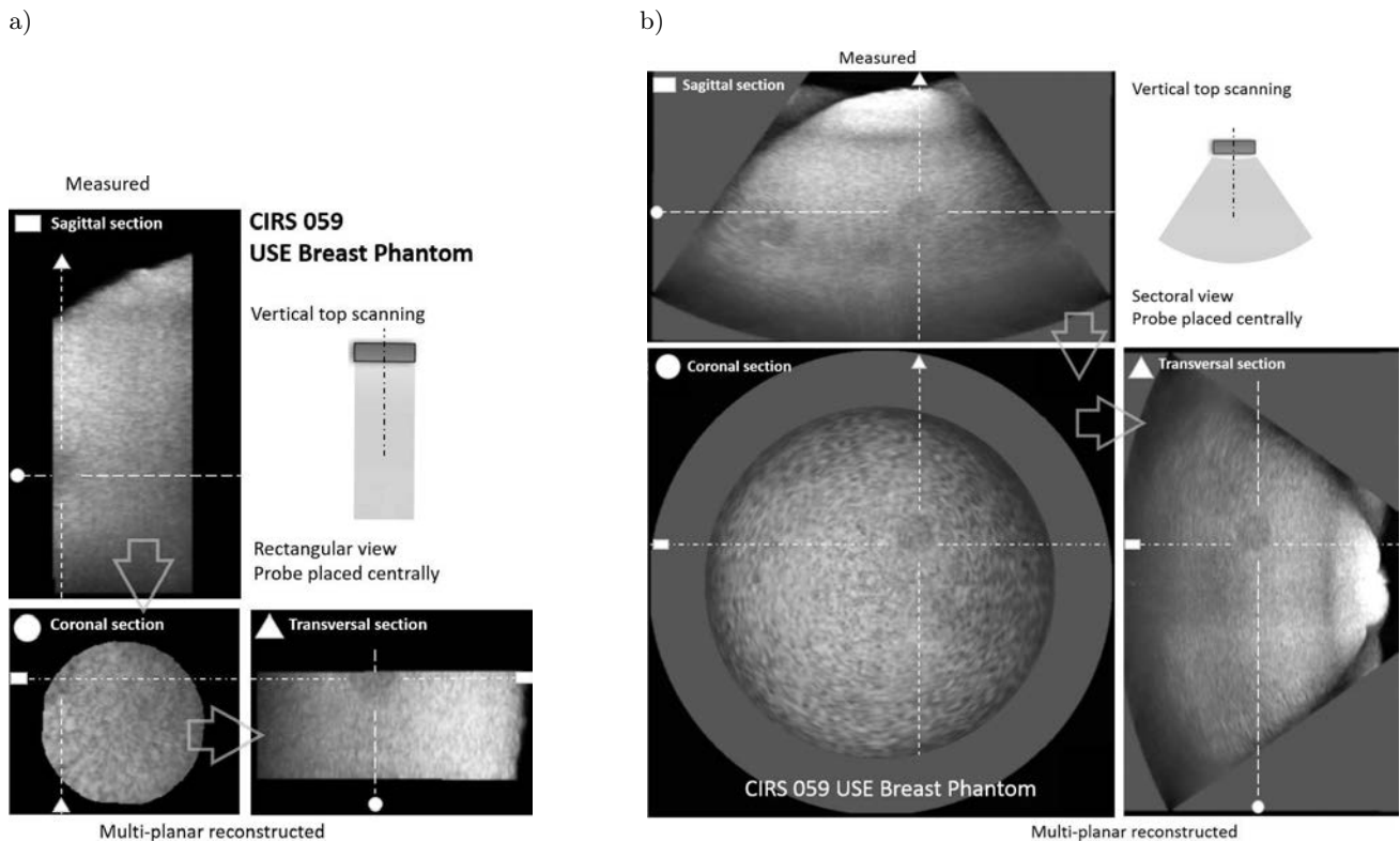
Fig. 13. Images of selected CIRS 059 USE breast phantom sections acquired using vertical top scanning with the probe placed centrally: a) rectangular view, b) sectoral view.
