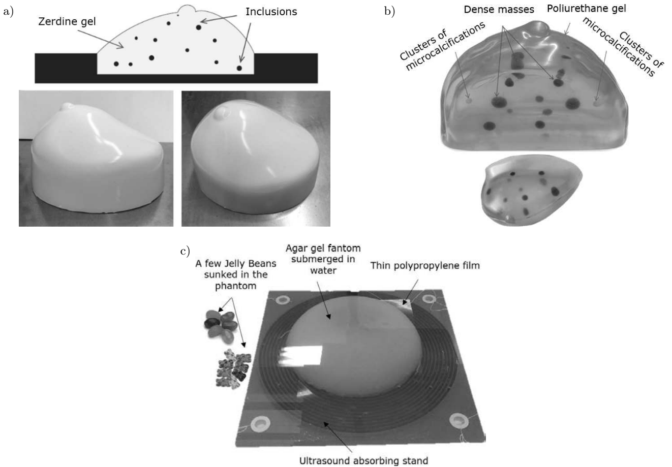
Fig. 7. Three different breast tissue phantoms used in the study: a) CIRS 059 USE Breast Phantom, b) CIRS 013 Mammography Breast Phantom, c) self-made US Agar Gel Phantom with sunken Jelly Beans.
