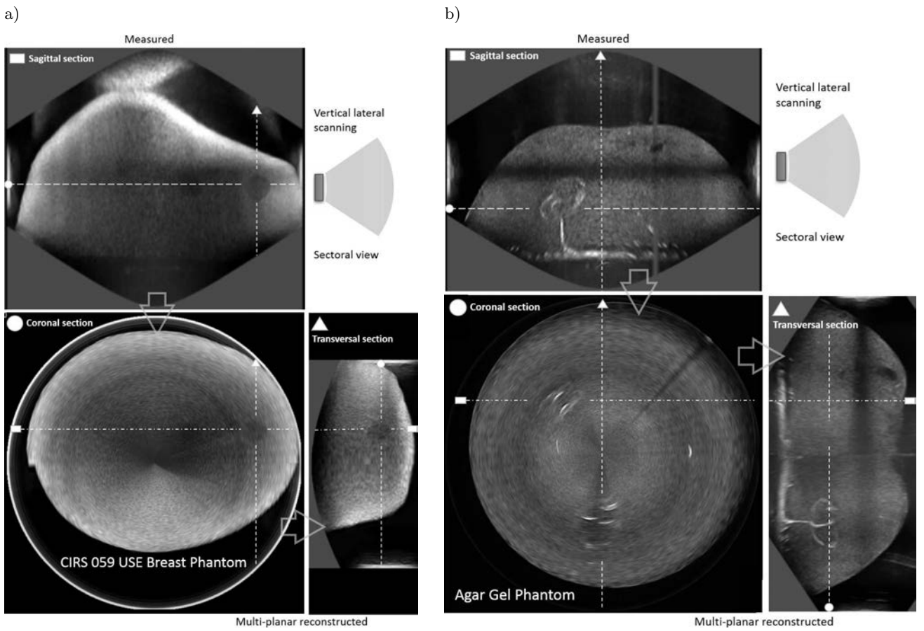
Fig. 12. Images of selected breast phantom sections acquired using vertical lateral scanning with the sectoral view: a) CIRS 059 USE Breast Phantom, b) US Agar Gel Phantom with sunken Jelly Beans.
