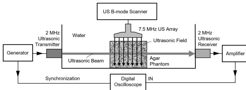
Fig. 16. The block scheme of the measurement setup to check the impact of ultrasonic fields in the ultrasound tomography scanning and the ultrasound echo scanning.
