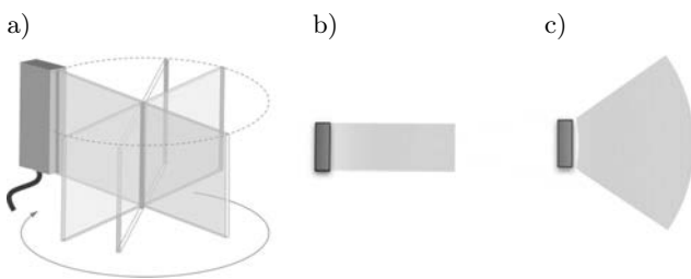
Fig. 9. The vertical lateral configuration applied in the MACUI method with different views: a) vertical lateral scanning, b) rectangular view, c) sectoral view.
