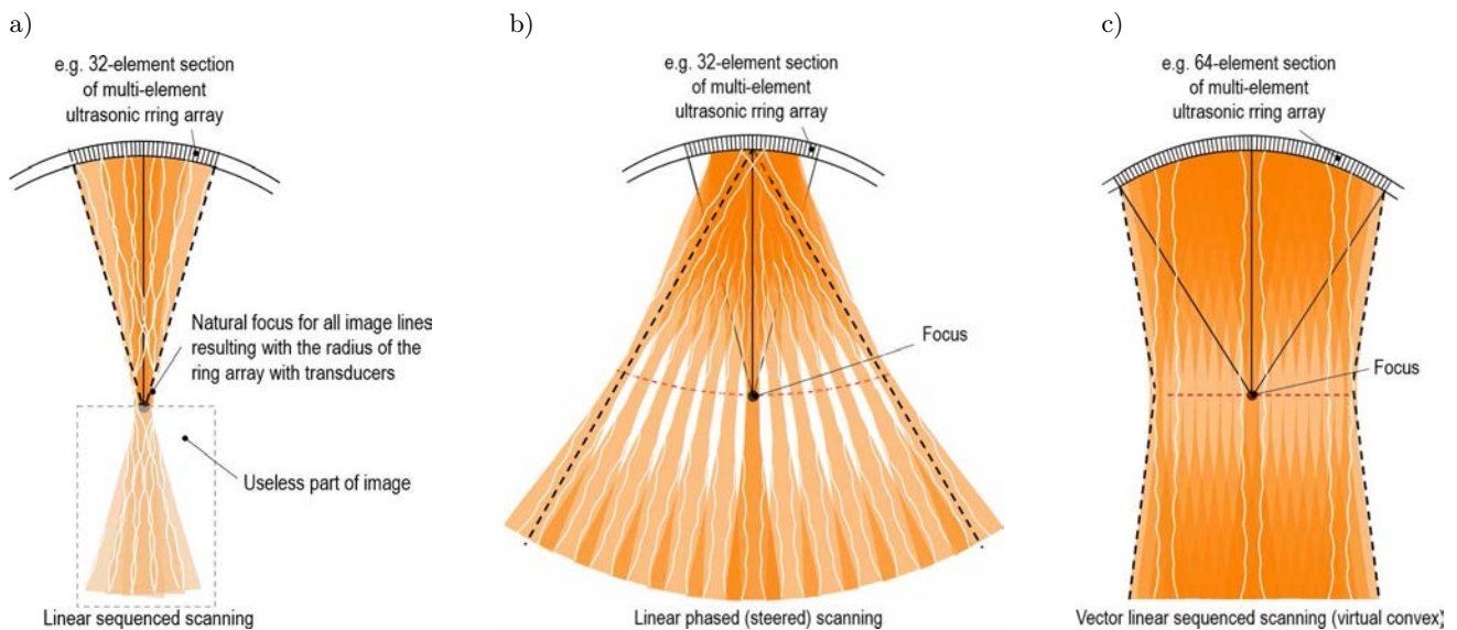
Fig. 1. US scanning methods which can be used by means of the specially designed ultrasound tomography multi-element ring array: a) linear sequenced scanning, b) linear phased (steered) scanning, c) vector linear scanning (so-called virtual convex).
