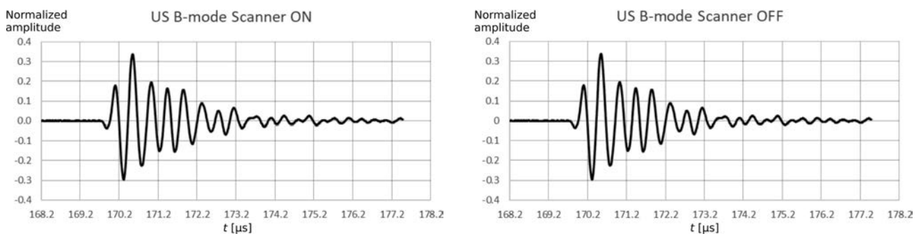
Fig. 17. The pulses transmitted through the medium as presented in Fig. 16 when the ultrasound B-mode scanner is ON and OFF.
