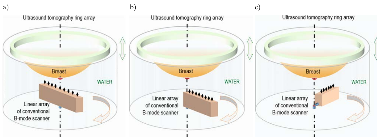
Fig. 3. Different multi-angle conventional ultrasound B-mode imaging (MACUI) methods designed as additional modality of developed prototype of ultrasound tomography scanner for in vivo female breast diagnosis, as an alternative to the FASCI method: a) with center of the additional linear array in the rotation axis, b) with edge of the additional linear array in the rotation axis, c) with edge of the additional linear array outside of the rotation axis.
