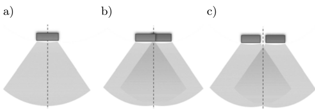
Fig. 10. Different positions of the probe for the tested vertical top configuration in the MACUI: a) centrally, b) 17 mm moved, c) 25 mm moved.
