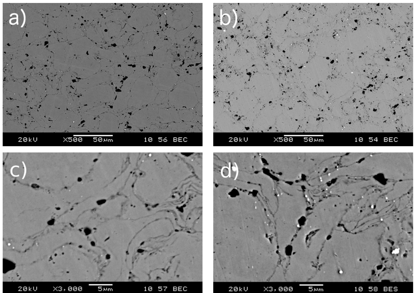
Fig. 7. Examples of microstructure images of the AISI 316L/ \text{TiB}_2/2\text{p} composites sintered by the HP-HT method: a) T = 900^\circ\text{C} , P = 5 \text{ GPa} , mag. 500\times ; b) T = 1300^\circ\text{C} , P = 5 \text{ GPa} , mag. 500\times ; c) T = 900^\circ\text{C} , P = 5 \text{ GPa} , mag. 3000\times ; d) T = 1300^\circ\text{C} , P = 5 \text{ GPa} , mag. 3000\times
