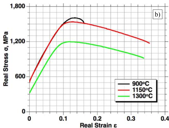
Fig. 4. Mechanical characteristics of the compression of samples after the HP-HT process conducted under conditions listed in Table 3: a) 5 GPa, b) 7 GPa
