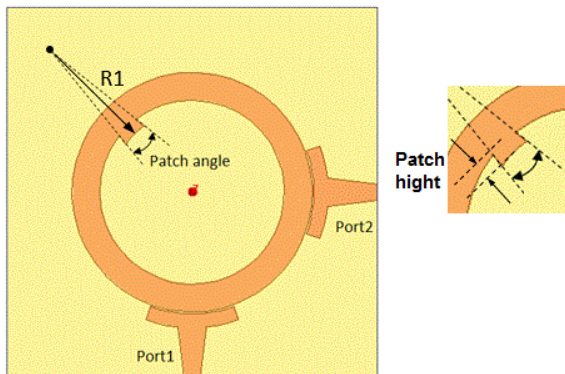
Fig. 11. Dual mode circular ring BPFs, perturbed by inner radial patch at azimuthal angle of 135^\circ . Main Dimensions are in (mm): R_{res} = 15.33 , R1 = 14.65 , wr = 3.33 , Notch-height = 1.28
