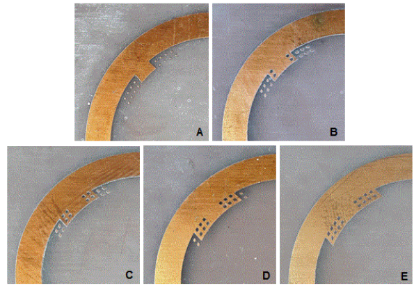
Fig. 15. Fabricated samples for the five cases of the perturbation element
