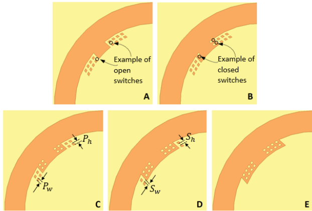
Fig. 13. Five cases of the designed patch (A,B,C,D,E) has different area, which modified by linking the different metallization by the switches
