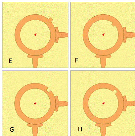
Fig. 8. Dual mode circular ring BPFs, perturbed by different cases of rectangular perturbation elements at azimuthal angles of 45°
