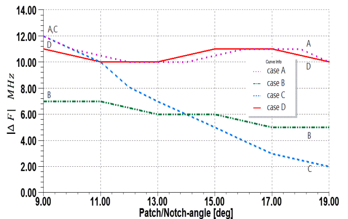
Fig. 9. Dual mode circular ring BPFs, perturbed by different cases of rectangular perturbation elements at azimuthal angles of 45°
