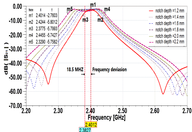
Fig. 4. Frequency responses ( |S_{21}| ) of the filter for several notch-depth values at notch angle equal to 12^\circ
