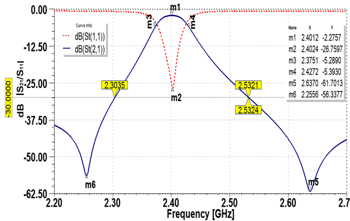
Fig. 3. Frequency responses ( |S_{21}| ), ( |S_{11}| ) of the filter circuit model with circuit parameters as given in Fig 2
