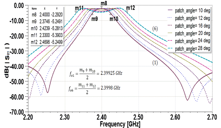
Fig. 12. Frequency responses ( |S_{21}| ) of the filter for several patch-angle values at notch depth equal to 1.25 mm
