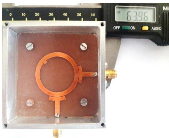
Fig. 14. Photograph of the fabricated filter for the case A of perturbation element
