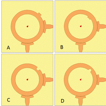
Fig. 7. Dual mode circular ring BPFs, perturbed by different cases of radial perturbation elements at azimuthal angles of 45°
