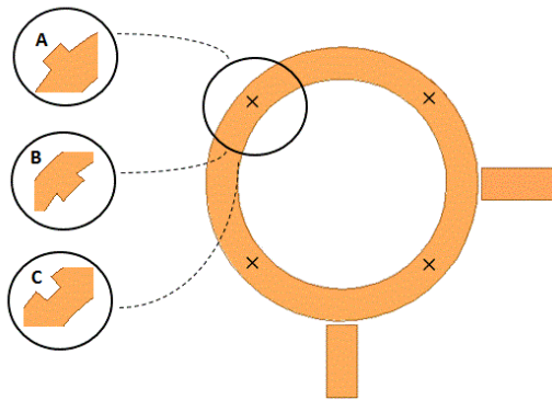
Fig. 1. Locations and shapes layout of perturbation element samples in circular ring dual mode BPF (x denotes suitable location, A: outer rectangular patch, B: inner radial patch, C: outer radial notch)
