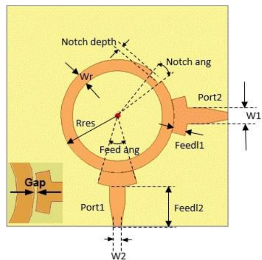
Fig. 2. Initially designed filter. Dimensions are in (mm): R_{res} = 15.3 , Gap = 0.2, Feed1 = 2.4, Feed2 = 11.8, w_1 = 3.5 , w_r = 3.21 , w_2 = 2 , Notch-depth = 1.28, Notch-ang = 12^\circ , Feed ang = 40^\circ
