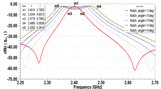
Fig. 6. Frequency responses ( |S_{21}| ) of the filter for several notch-angle values at notch depth to 1.2 mm
