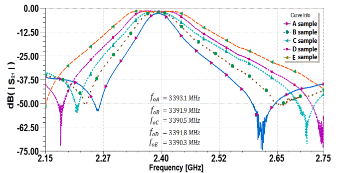
Fig. 17. Measured frequency responses ( |S_{21}| ) of the implemented filters
