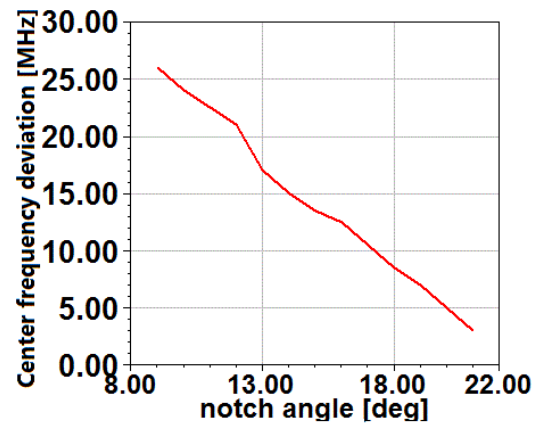
Fig. 5. Center frequency deviation for several values of notch angle for FBW increase equal to [3:1]
