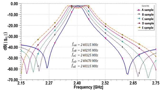
Fig. 16. Frequency responses ( |S_{21}| ) of the designed filter for five samples of patch size
