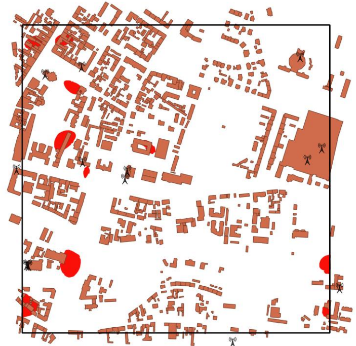
Fig. 8. Visualization of an example flat 2D electromagnetic field strength distribution for the selected exceeded limit value of (7 V/m) for a height range of 0.3-2 m a.s.l. at a map including a plane buildings (BDOT10K). Places with estimated values > 7 V/m are marked in red.
