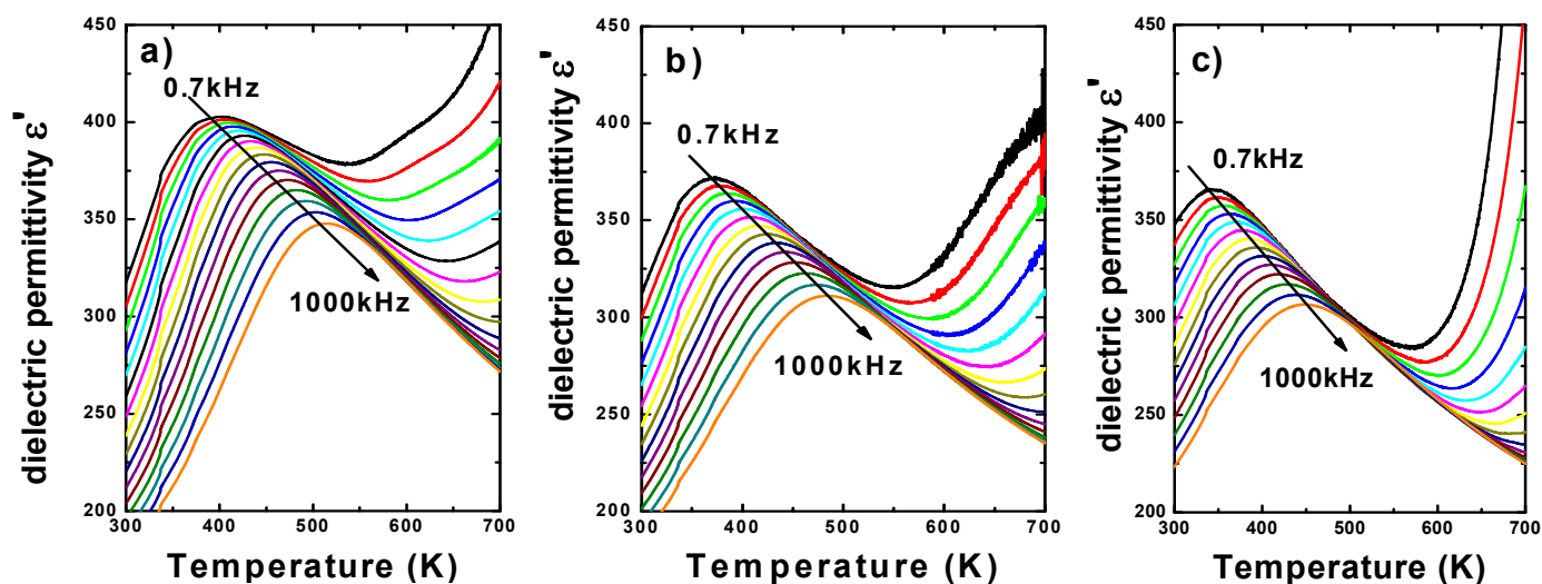
Fig. 4. Real part of dielectric permittivity as a function of temperature measured on heating at various frequencies of measuring field, for undoped BBN (a), BBN+1 at. %La (b) and BBN+5 at. %La (c) ceramics
