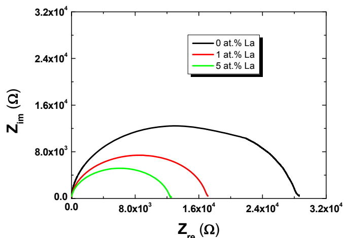
Fig. 6. Nyquist plot for BBN ceramics pure and La-doped obtained at temperature 723 K
