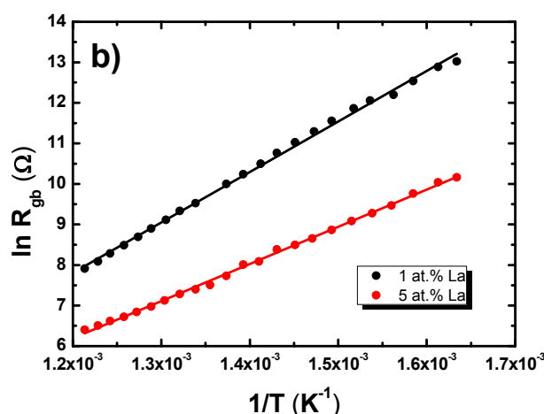
Fig. 8. Arrhenius plots for calculation of conduction activation energies of grain (a) and grain boundary (b)
