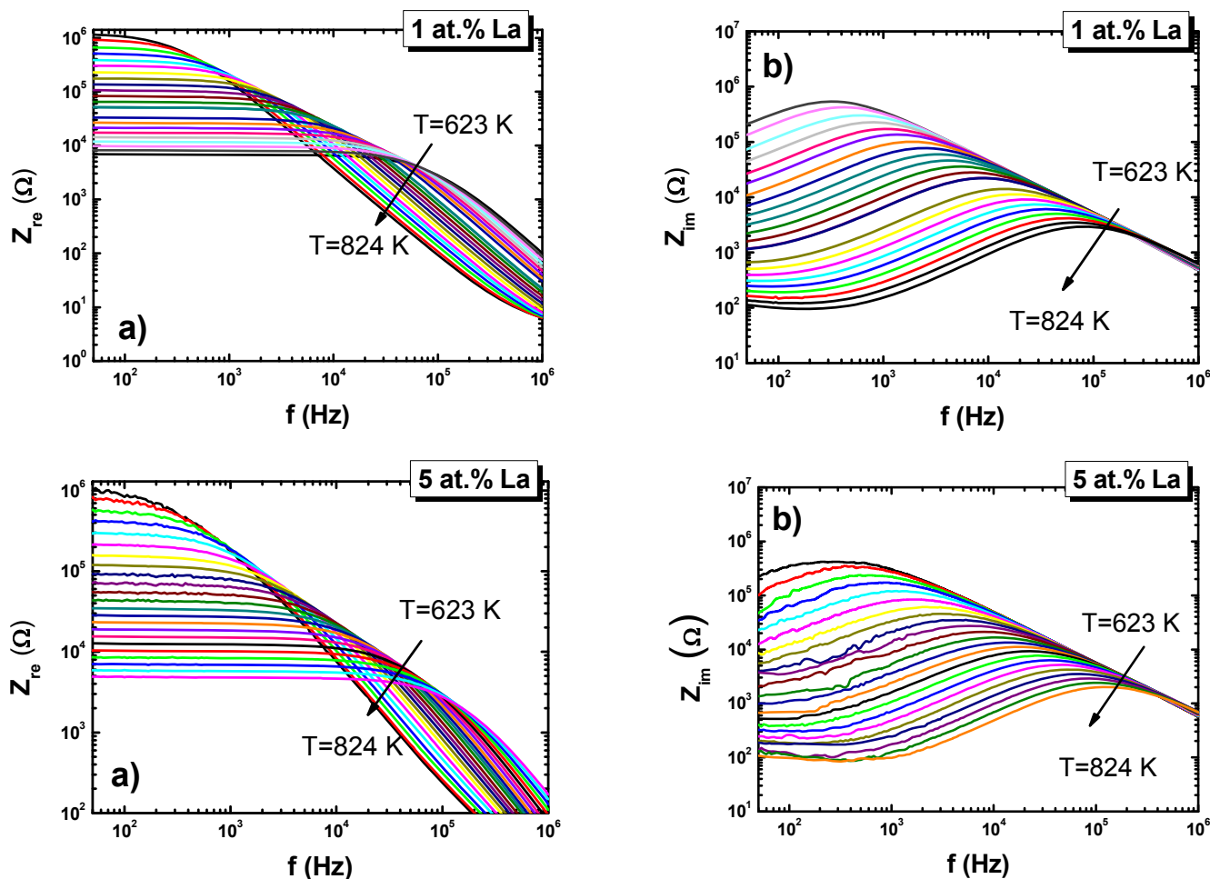
Fig. 5. The frequency dependence of real part (a) and imaginary (b) of the impedance at various temperature for BBN ceramics modified with lanthanum
