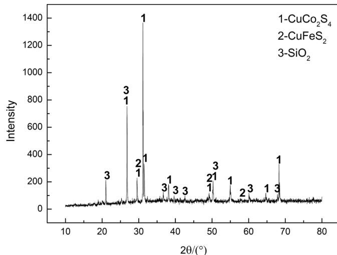
Fig. 1. The X-ray diffraction pattern of carrollite ore
