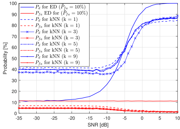
Fig. 4. Results of kNN algorithm for \bar{P}_{fa} = 10\% .
