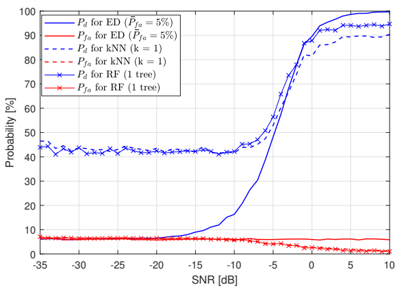
Fig. 8. Results of kNN and RF algorithms for \bar{P}_{fa} = 5\% .
