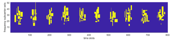
Fig. 1. Sample LTE resources allocation in time and frequency.
