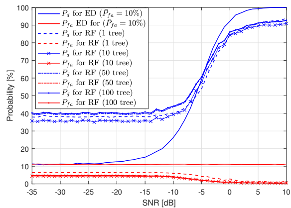
Fig. 6. Results of RF algorithm for \bar{P}_{fa} = 10\% .
