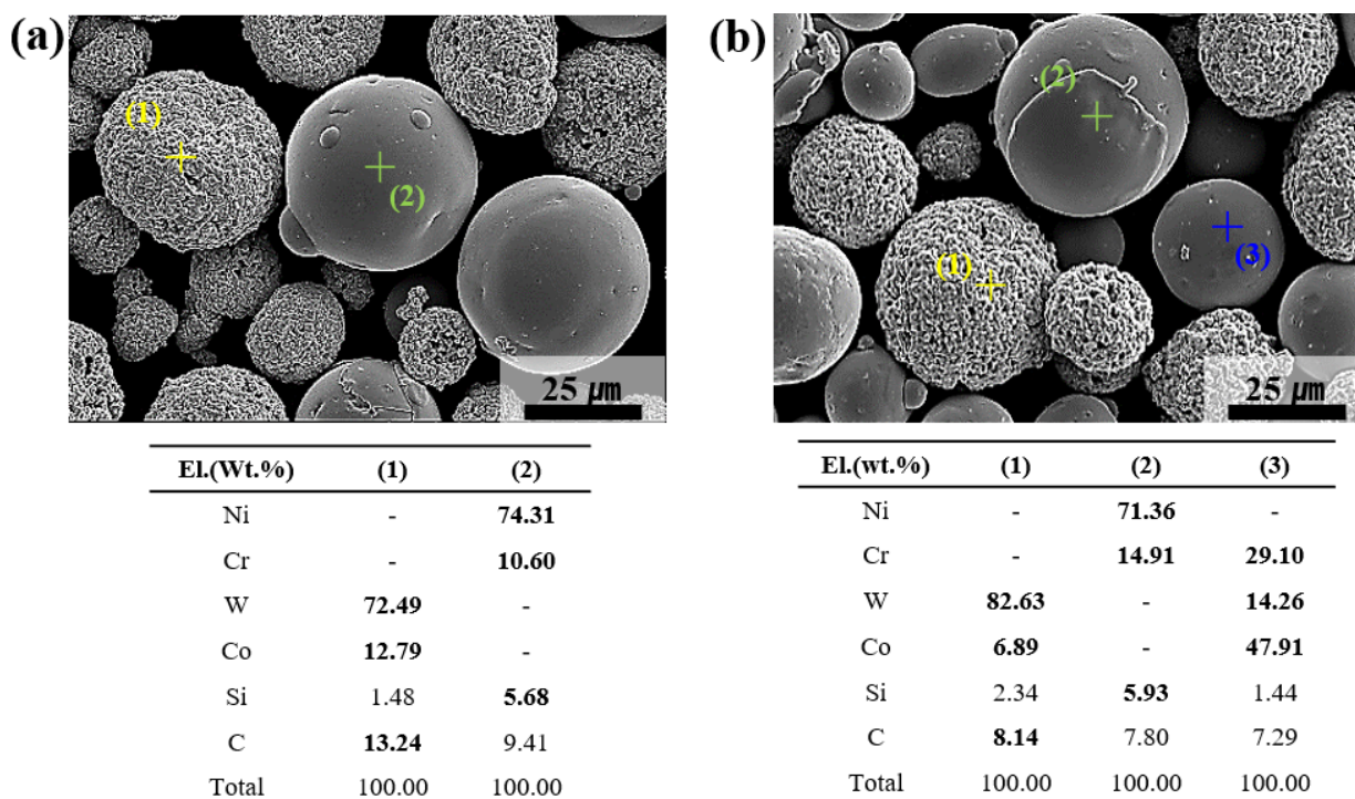
Fig. 1. Morphologies of initial powders used in this study; (a) WC-50Ni and (b) WC-50Ni+ST1
