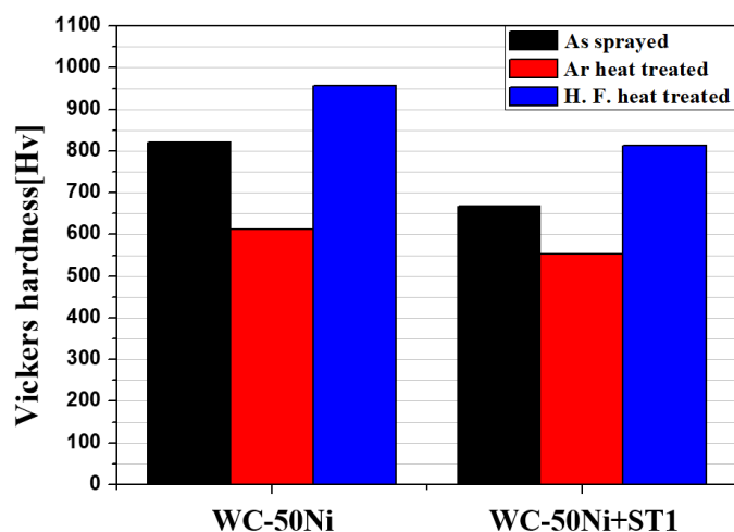
Fig. 7. Vickers hardness results of WC-50Ni and WC-50Ni+ST1 coating layers
