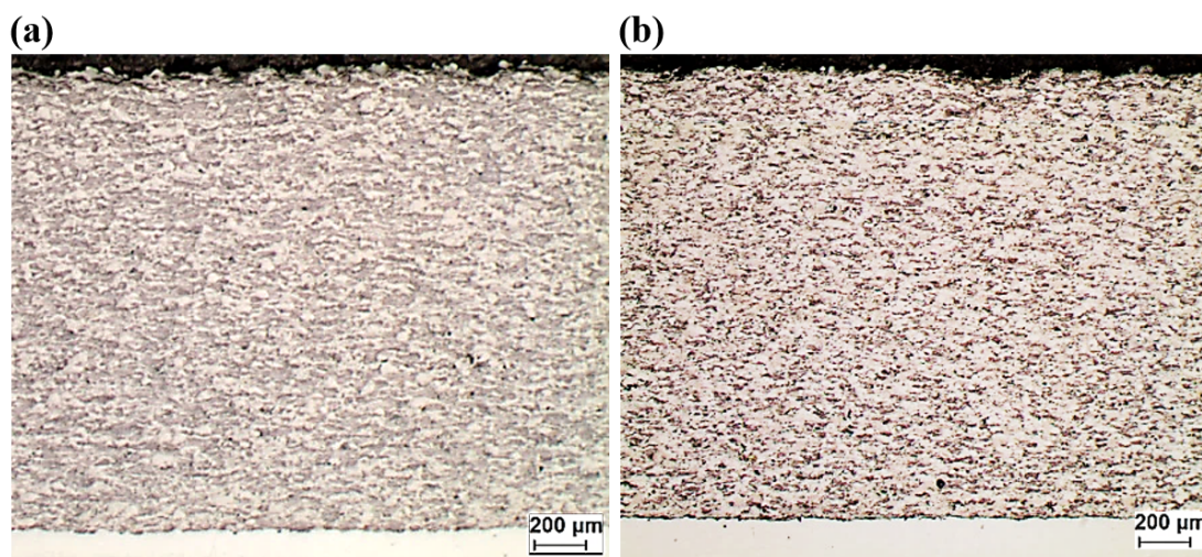
Fig. 3. Macroscopic images of as sprayed coating layers; (a) WC-50Ni and (b) WC-50Ni+ST1
