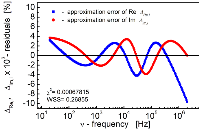
Fig. 7. Fit-quality plot for CNLS-fit of experimental impedance data and Voigt's model
