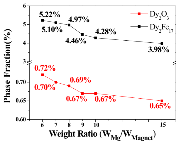
Fig. 6. Fraction of Dy-oxide and Dy_2Fe_{17} with Mg ratio using image analysis
