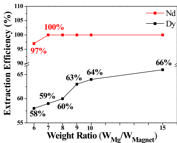
Fig. 7. Extraction efficiency of rare earths
