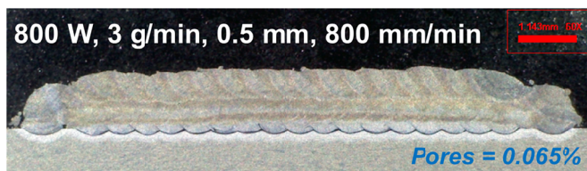
Fig. 6. Multi-layered deposition of the HTCS-150 with the minimum pores and no lack of fusion
