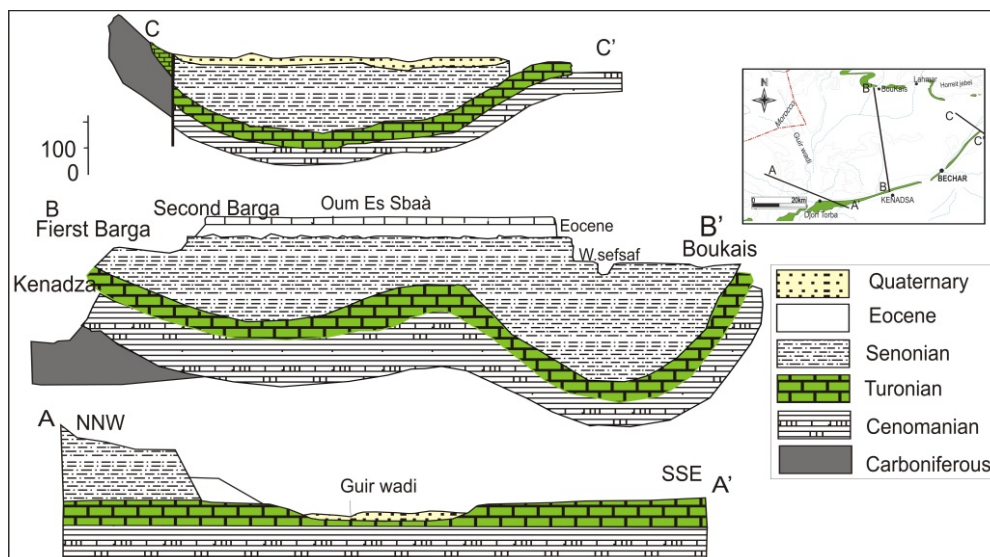
Fig. 2. Interactive hydrogeological cross section of the Turonian aquifer; source: IDROTECNECO [1976], modified
