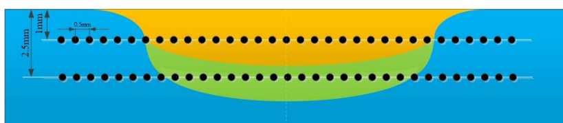
Fig. 3. Schematic of measurement points of the microhardness test
