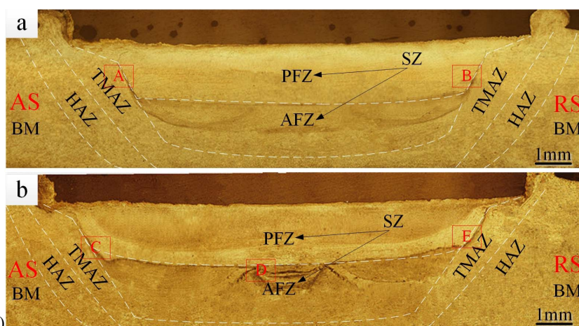
Fig. 5. Macrostructures of the repaired joints using two welding processes: (a) ultrasonic assisted A-PFFSR and (b) conventional A-PFFSR
